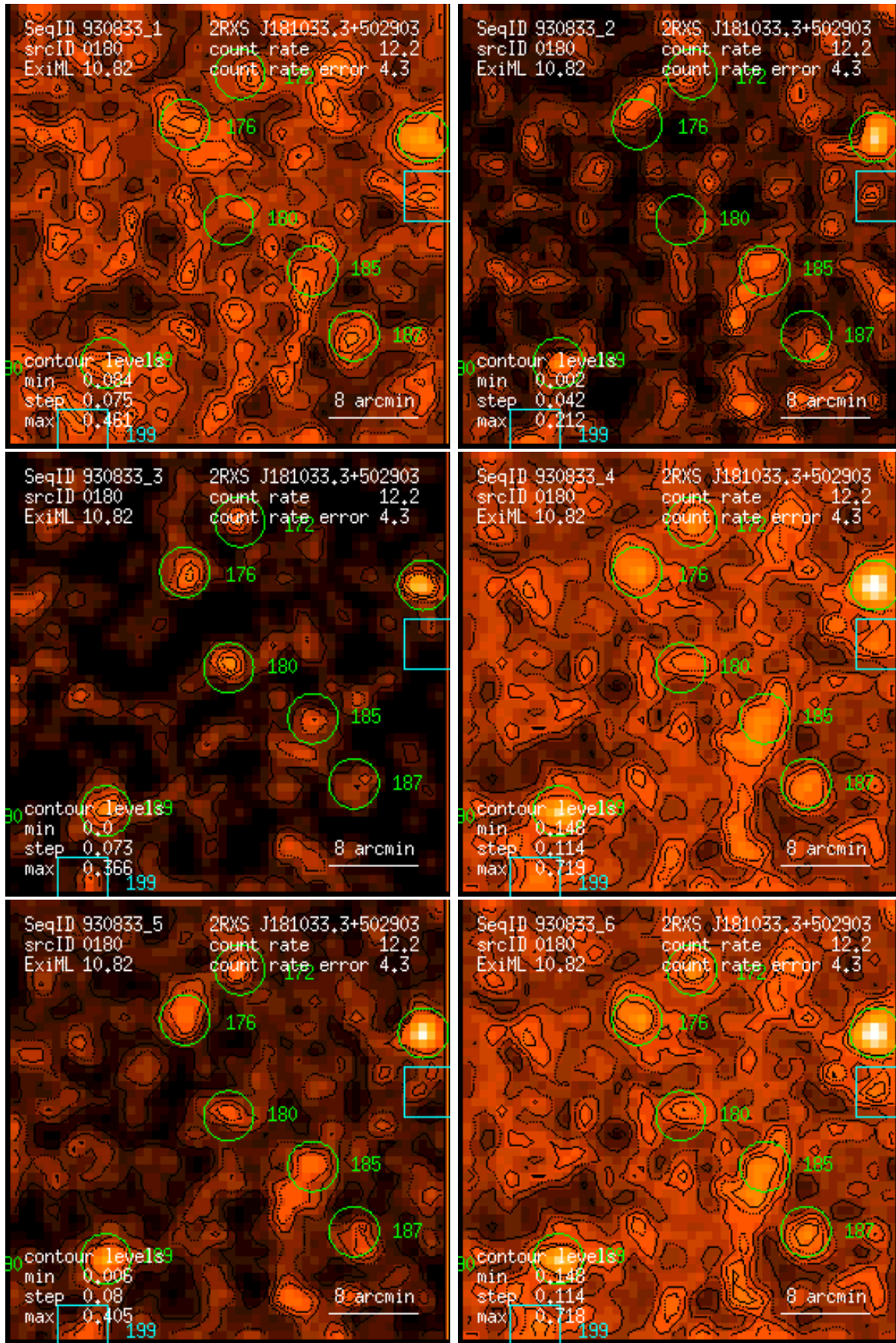
Figure 180: RASS 930833: detection 0180: band rate images, Gaussian filter: (1) PSPC channels 11 – 41, (2) 52 – 90, (3) 91 – 201, (4) 11 – 235, (5) 52 – 201, (6) 11 – 201. Broad band rates in counts/ks. Band rate contour levels in counts/ks/arcmin 2 .
