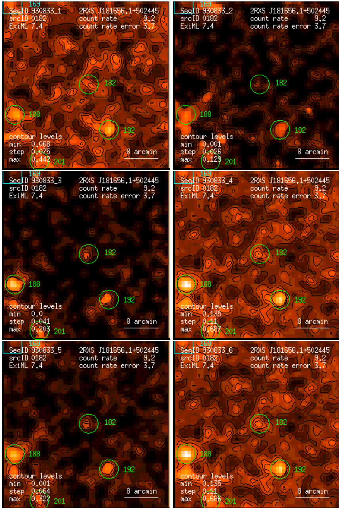
Figure 182: RASS 930833: detection 0182: band rate images, Gaussian filter: (1) PSPC channels 11 – 41, (2) 52 – 90, (3) 91 – 201, (4) 11 – 235, (5) 52 – 201, (6) 11 – 201. Broad band rates in counts/ks. Band rate contour levels in counts/ks/arcmin 2 .
