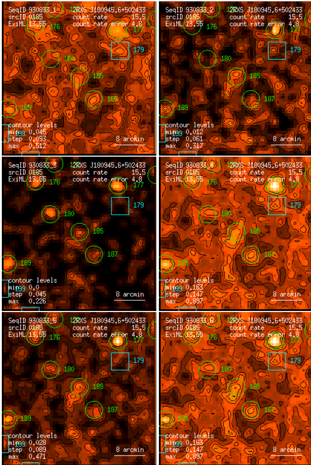
Figure 185: RASS 930833: detection 0185: band rate images, Gaussian filter: (1) PSPC channels 11 – 41, (2) 52 – 90, (3) 91 – 201, (4) 11 – 235, (5) 52 – 201, (6) 11 – 201. Broad band rates in counts/ks. Band rate contour levels in counts/ks/arcmin 2 .
