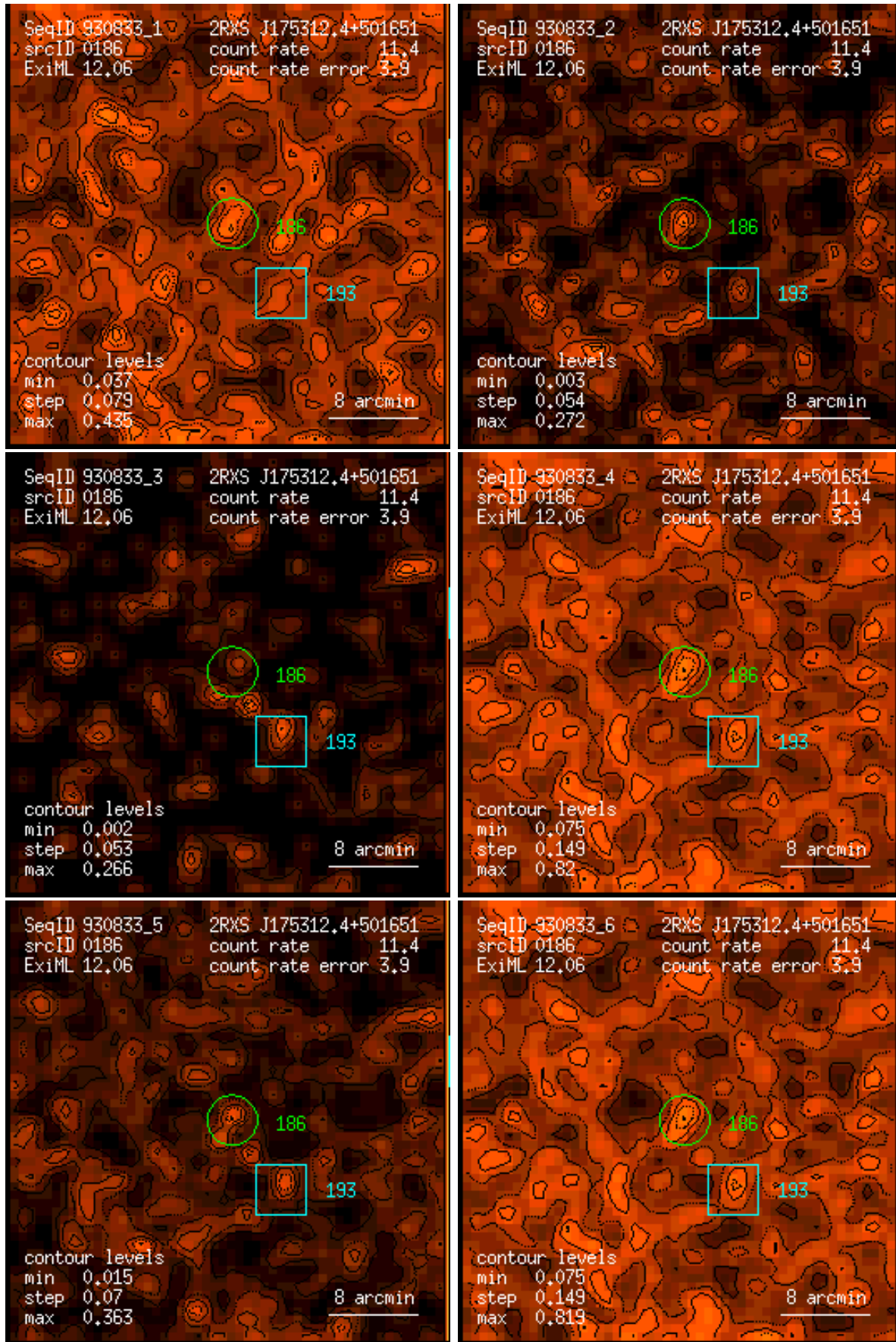
Figure 186: RASS 930833: detection 0186: band rate images, Gaussian filter: (1) PSPC channels 11 – 41, (2) 52 – 90, (3) 91 – 201, (4) 11 – 235, (5) 52 – 201, (6) 11 – 201. Broad band rates in counts/ks. Band rate contour levels in counts/ks/arcmin 2 .
