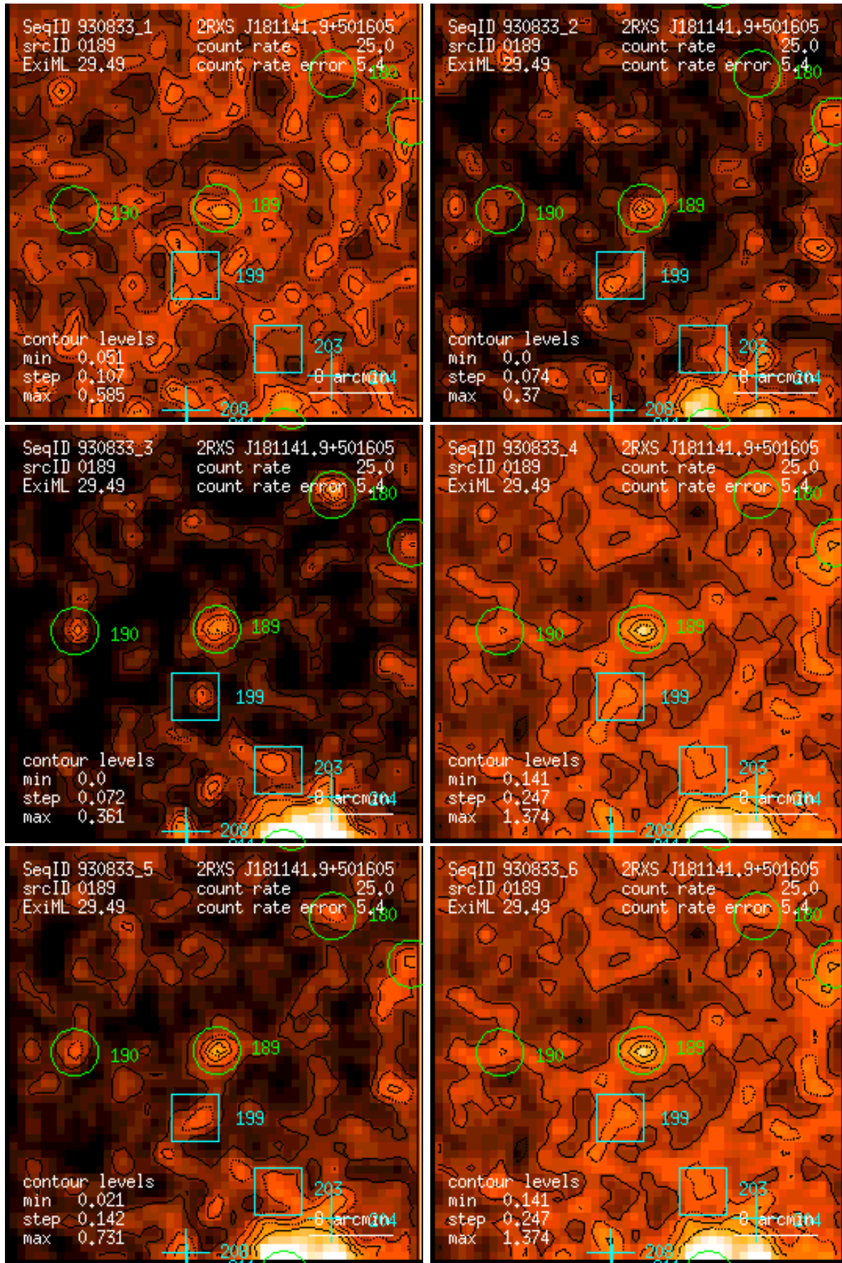
Figure 189: RASS 930833: detection 0189: band rate images, Gaussian filter: (1) PSPC channels 11 – 41, (2) 52 – 90, (3) 91 – 201, (4) 11 – 235, (5) 52 – 201, (6) 11 – 201. Broad band rates in counts/ks. Band rate contour levels in counts/ks/arcmin 2 .
