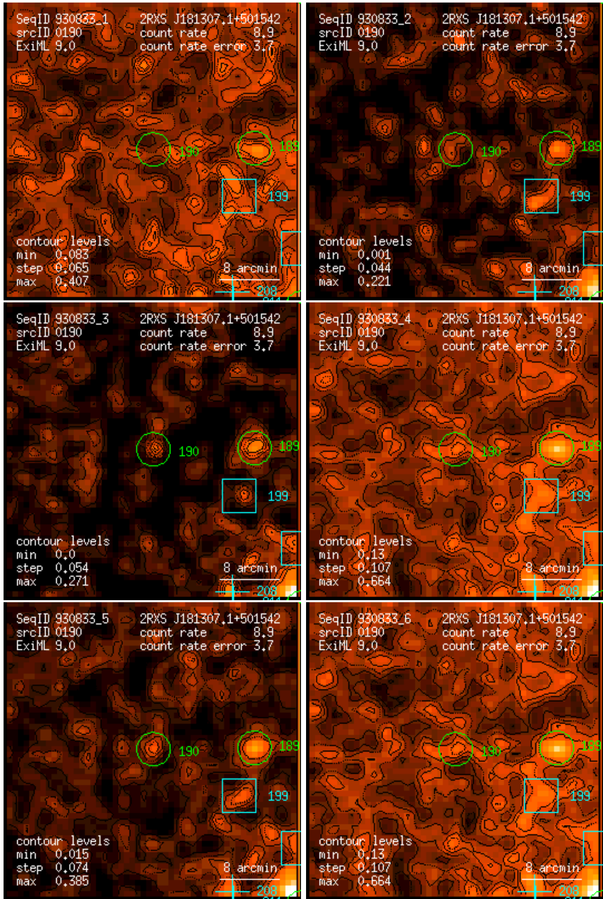
Figure 190: RASS 930833: detection 0190: band rate images, Gaussian filter: (1) PSPC channels 11 – 41, (2) 52 – 90, (3) 91 – 201, (4) 11 – 235, (5) 52 – 201, (6) 11 – 201. Broad band rates in counts/ks. Band rate contour levels in counts/ks/arcmin 2 .
