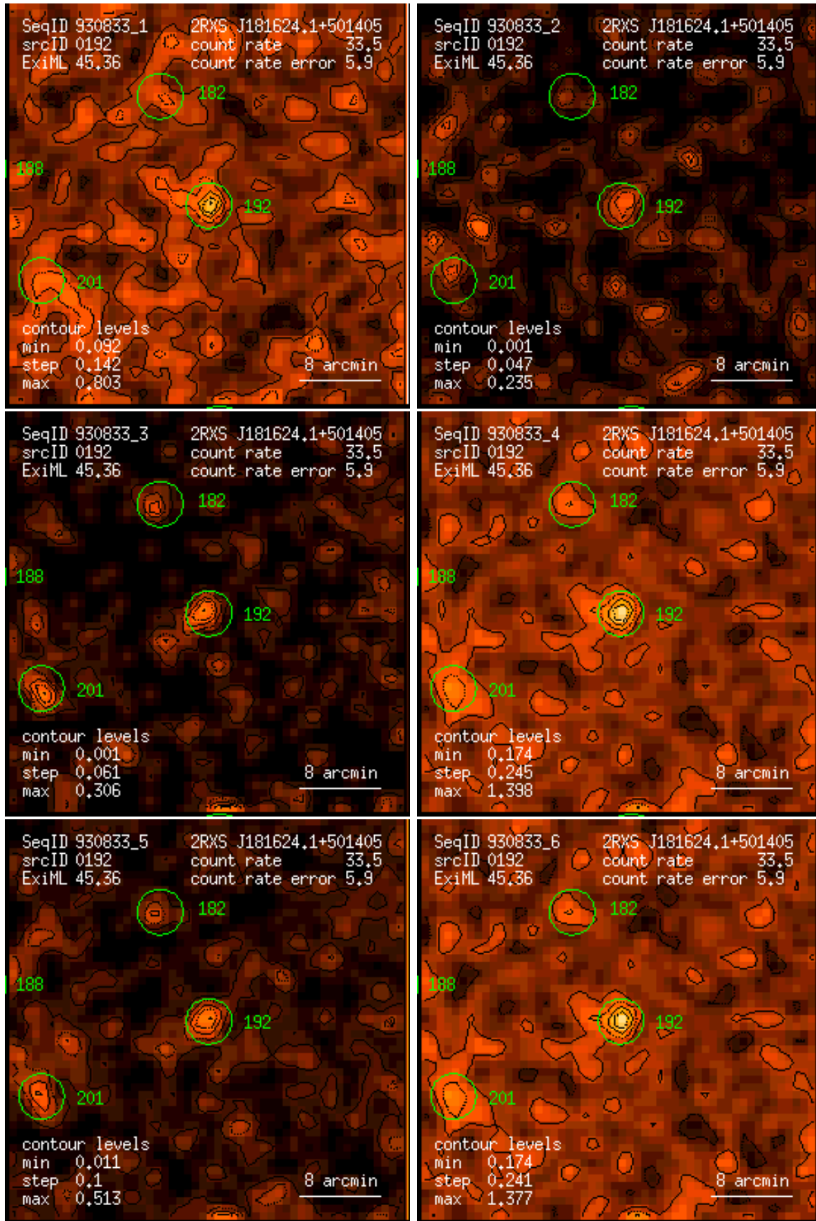
Figure 192: RASS 930833: detection 0192: band rate images, Gaussian filter: (1) PSPC channels 11 – 41, (2) 52 – 90, (3) 91 – 201, (4) 11 – 235, (5) 52 – 201, (6) 11 – 201. Broad band rates in counts/ks. Band rate contour levels in counts/ks/arcmin 2 .
