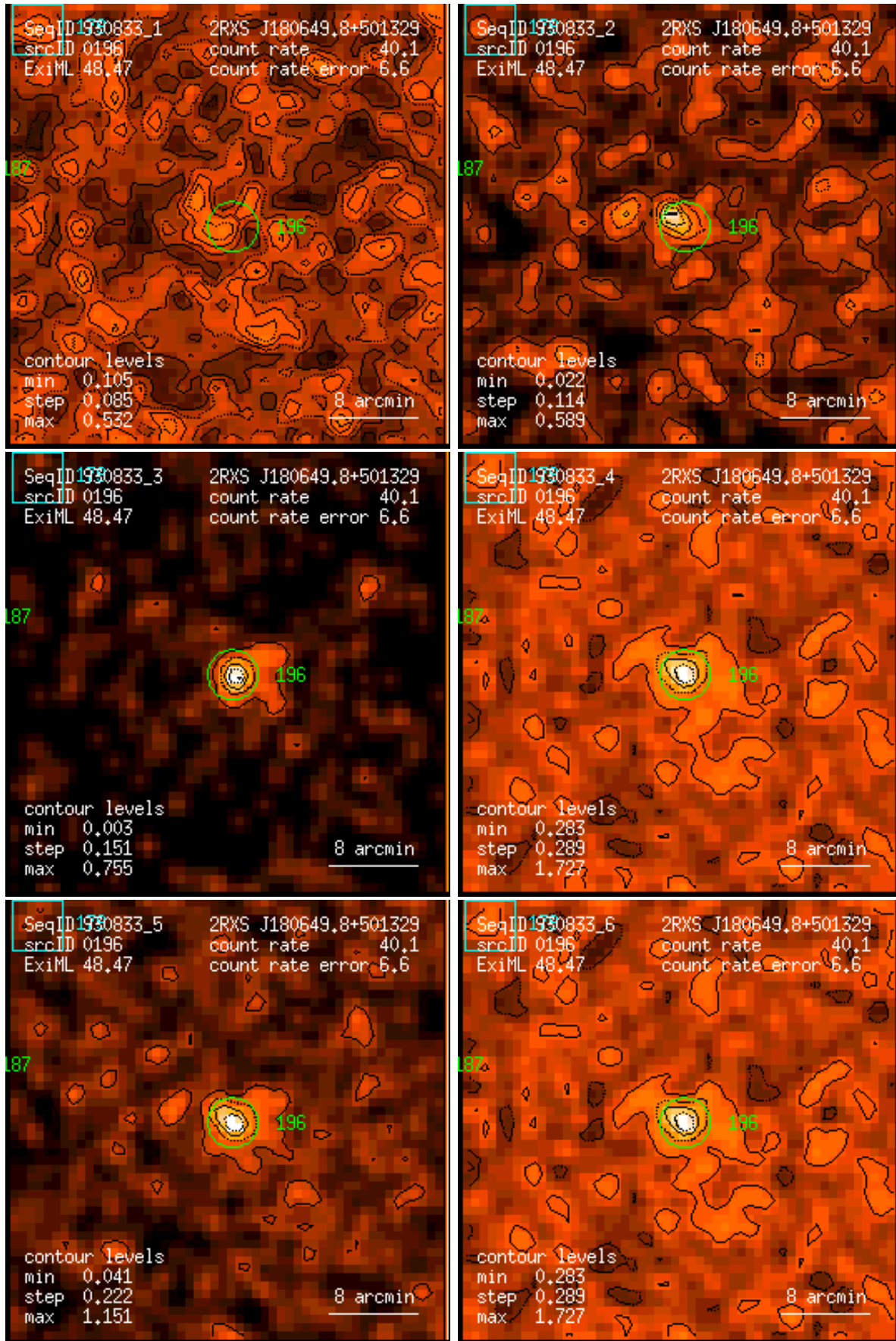
Figure 196: RASS 930833: detection 0196: band rate images, Gaussian filter: (1) PSPC channels 11 – 41, (2) 52 – 90, (3) 91 – 201, (4) 11 – 235, (5) 52 – 201, (6) 11 – 201. Broad band rates in counts/ks. Band rate contour levels in counts/ks/arcmin 2 .
