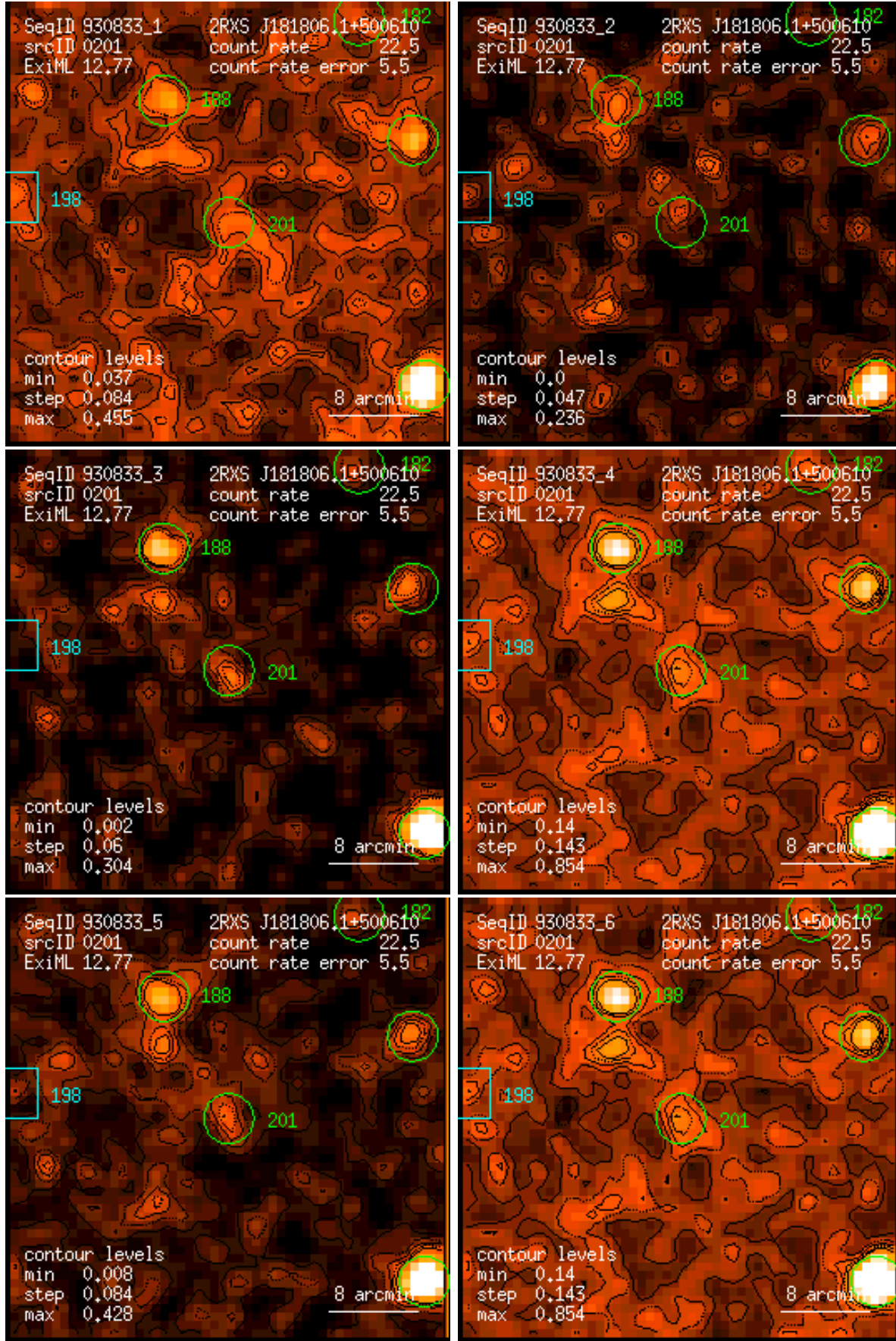
Figure 201: RASS 930833: detection 0201: band rate images, Gaussian filter: (1) PSPC channels 11 – 41, (2) 52 – 90, (3) 91 – 201, (4) 11 – 235, (5) 52 – 201, (6) 11 – 201. Broad band rates in counts/ks. Band rate contour levels in counts/ks/arcmin 2 .
