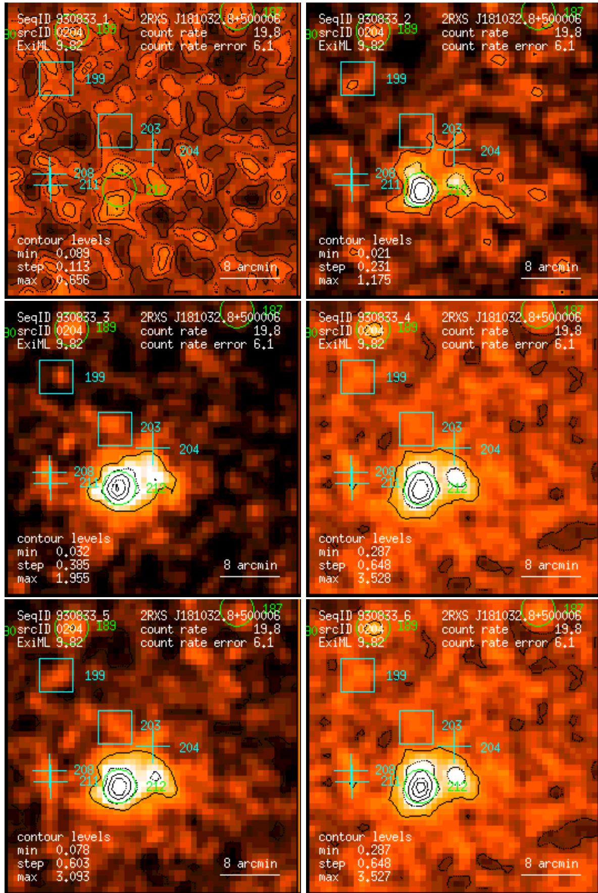
Figure 204: RASS 930833: detection 0204: band rate images, Gaussian filter: (1) PSPC channels 11 – 41, (2) 52 – 90, (3) 91 – 201, (4) 11 – 235, (5) 52 – 201, (6) 11 – 201. Broad band rates in counts/ks. Band rate contour levels in counts/ks/arcmin 2 .
