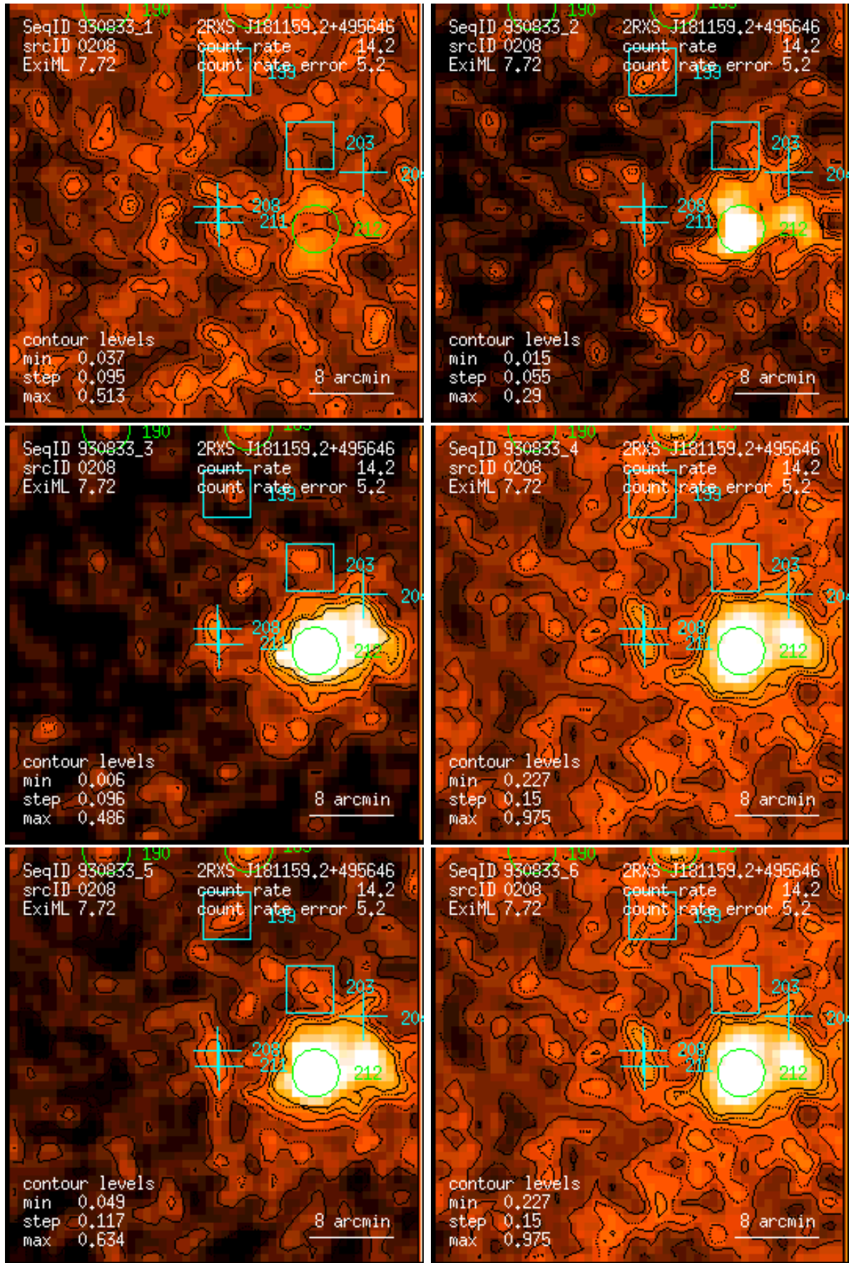
Figure 208: RASS 930833: detection 0208: band rate images, Gaussian filter: (1) PSPC channels 11 – 41, (2) 52 – 90, (3) 91 – 201, (4) 11 – 235, (5) 52 – 201, (6) 11 – 201. Broad band rates in counts/ks. Band rate contour levels in counts/ks/arcmin 2 .
