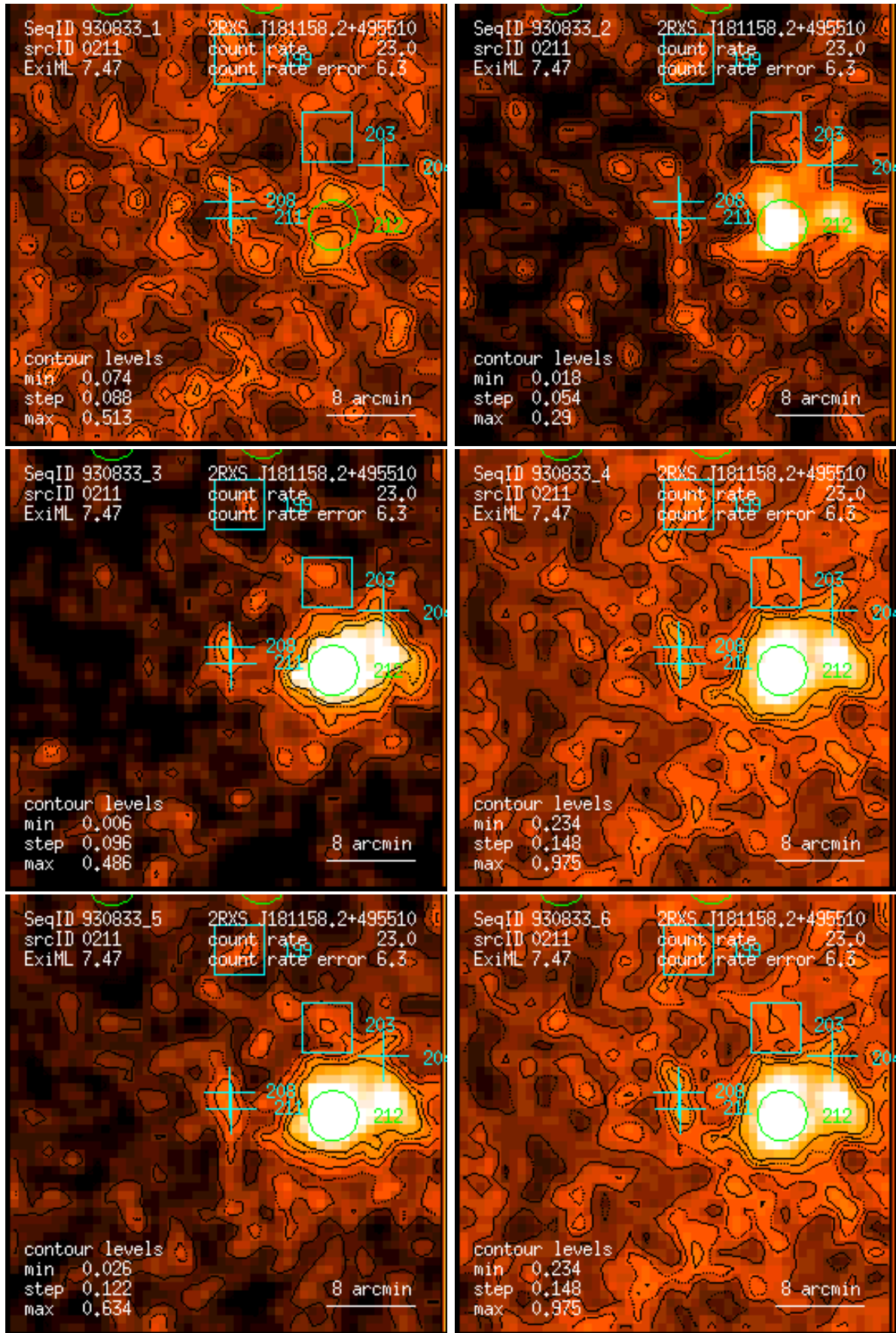
Figure 211: RASS 930833: detection 0211: band rate images, Gaussian filter: (1) PSPC channels 11 – 41, (2) 52 – 90, (3) 91 – 201, (4) 11 – 235, (5) 52 – 201, (6) 11 – 201. Broad band rates in counts/ks. Band rate contour levels in counts/ks/arcmin 2 .
