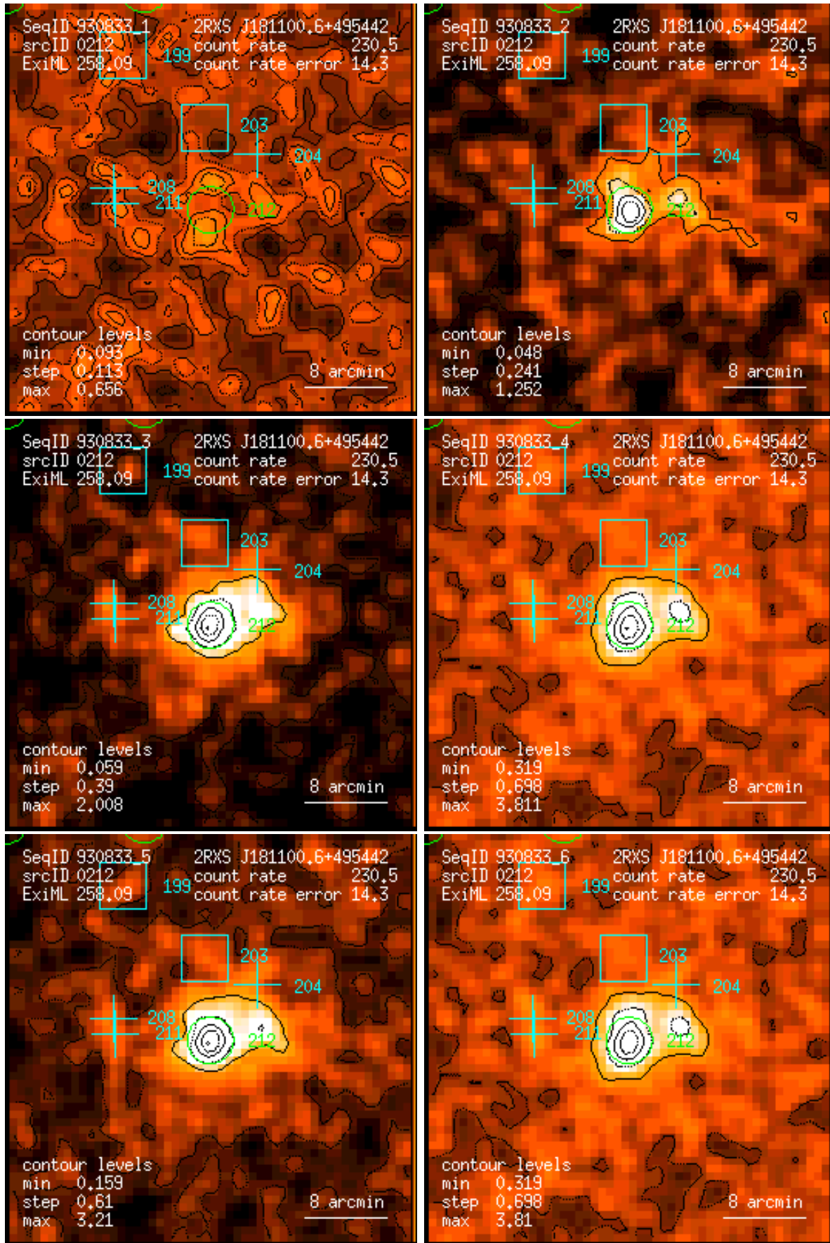
Figure 212: RASS 930833: detection 0212: band rate images, Gaussian filter: (1) PSPC channels 11 – 41, (2) 52 – 90, (3) 91 – 201, (4) 11 – 235, (5) 52 – 201, (6) 11 – 201. Broad band rates in counts/ks. Band rate contour levels in counts/ks/arcmin 2 .
