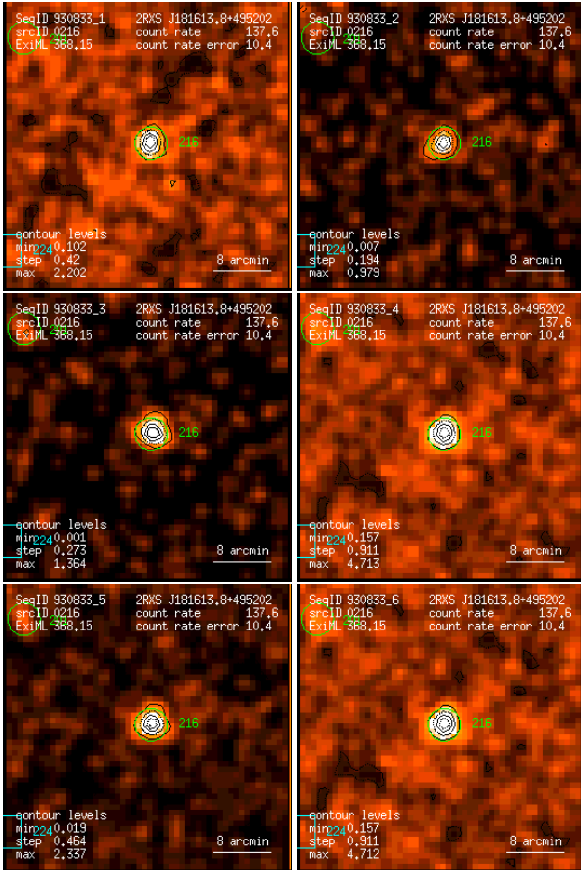
Figure 216: RASS 930833: detection 0216: band rate images, Gaussian filter: (1) PSPC channels 11 – 41, (2) 52 – 90, (3) 91 – 201, (4) 11 – 235, (5) 52 – 201, (6) 11 – 201. Broad band rates in counts/ks. Band rate contour levels in counts/ks/arcmin 2 .
