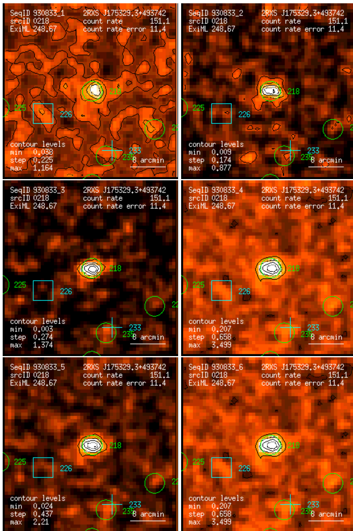
Figure 218: RASS 930833: detection 0218: band rate images, Gaussian filter: (1) PSPC channels 11 – 41, (2) 52 – 90, (3) 91 – 201, (4) 11 – 235, (5) 52 – 201, (6) 11 – 201. Broad band rates in counts/ks. Band rate contour levels in counts/ks/arcmin 2 .
