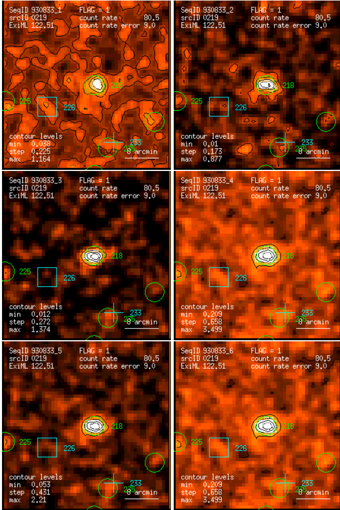
Figure 219: RASS 930833: detection 0219: band rate images, Gaussian filter: (1) PSPC channels 11 – 41, (2) 52 – 90, (3) 91 – 201, (4) 11 – 235, (5) 52 – 201, (6) 11 – 201. Broad band rates in counts/ks. Band rate contour levels in counts/ks/arcmin 2 .
