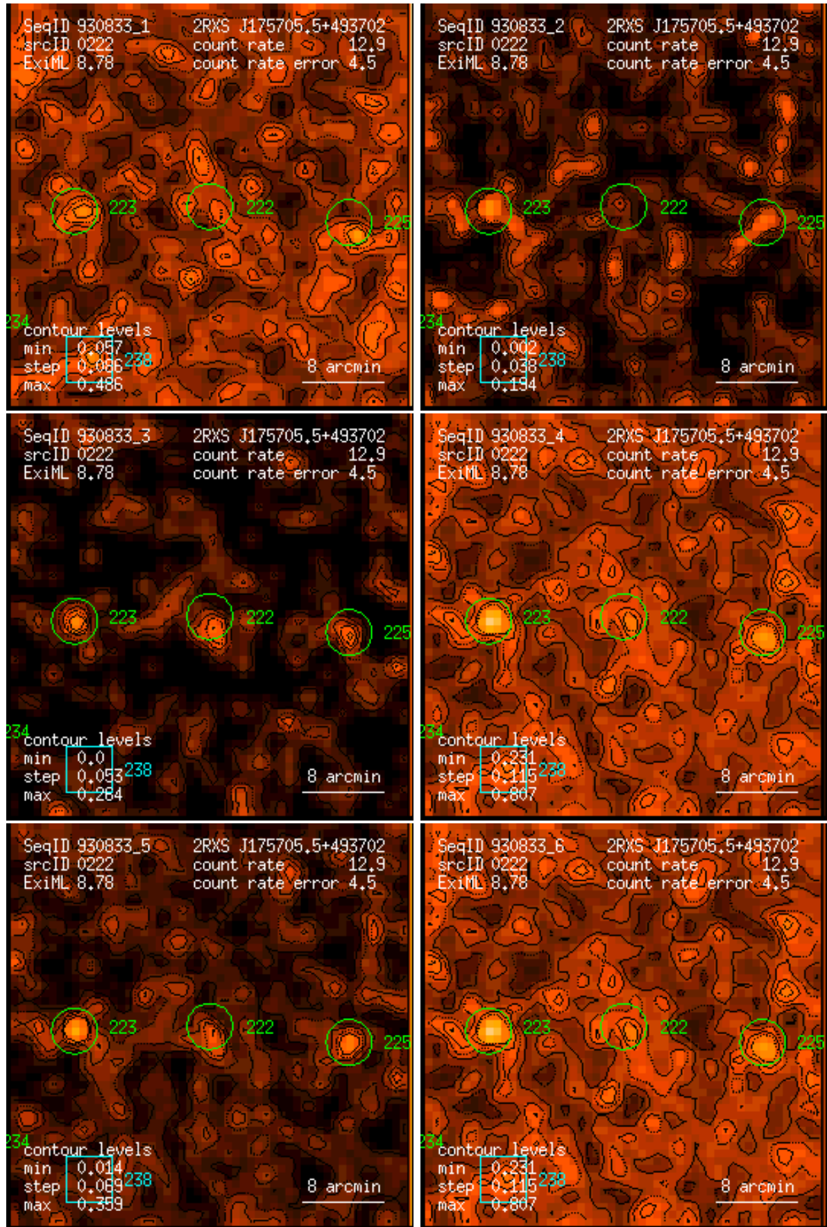
Figure 222: RASS 930833: detection 0222: band rate images, Gaussian filter: (1) PSPC channels 11 – 41, (2) 52 – 90, (3) 91 – 201, (4) 11 – 235, (5) 52 – 201, (6) 11 – 201. Broad band rates in counts/ks. Band rate contour levels in counts/ks/arcmin 2 .
