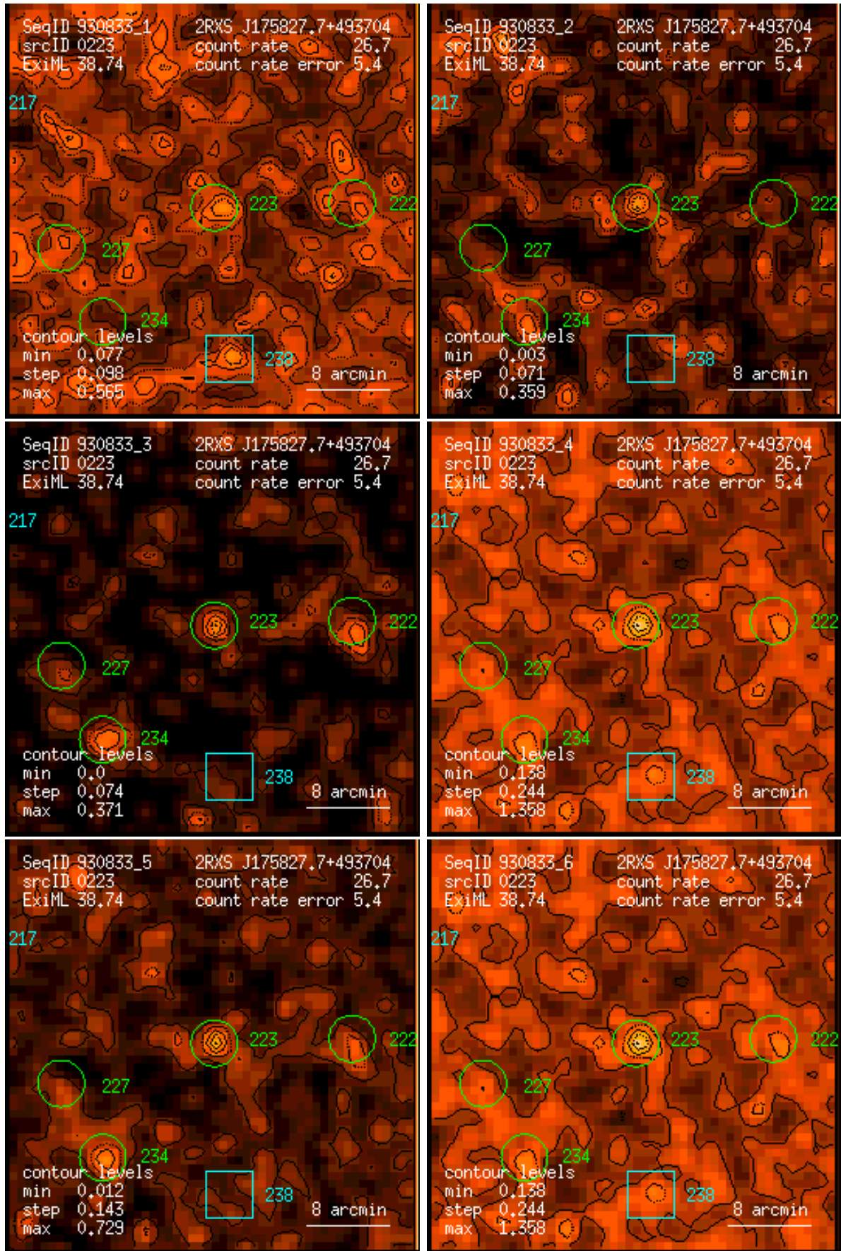
Figure 223: RASS 930833: detection 0223: band rate images, Gaussian filter: (1) PSPC channels 11 – 41, (2) 52 – 90, (3) 91 – 201, (4) 11 – 235, (5) 52 – 201, (6) 11 – 201. Broad band rates in counts/ks. Band rate contour levels in counts/ks/arcmin 2 .
