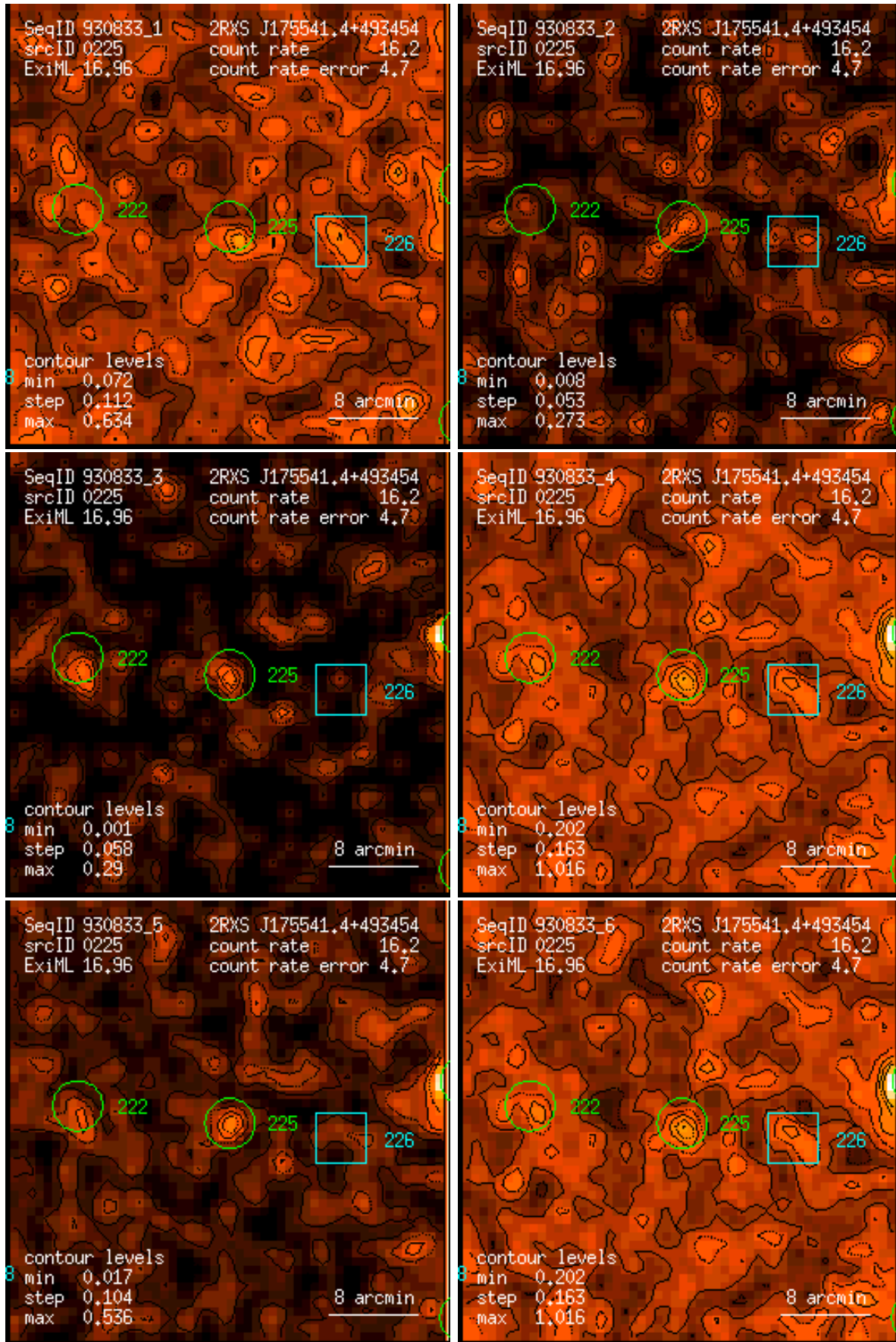
Figure 225: RASS 930833: detection 0225: band rate images, Gaussian filter: (1) PSPC channels 11 – 41, (2) 52 – 90, (3) 91 – 201, (4) 11 – 235, (5) 52 – 201, (6) 11 – 201. Broad band rates in counts/ks. Band rate contour levels in counts/ks/arcmin 2 .
