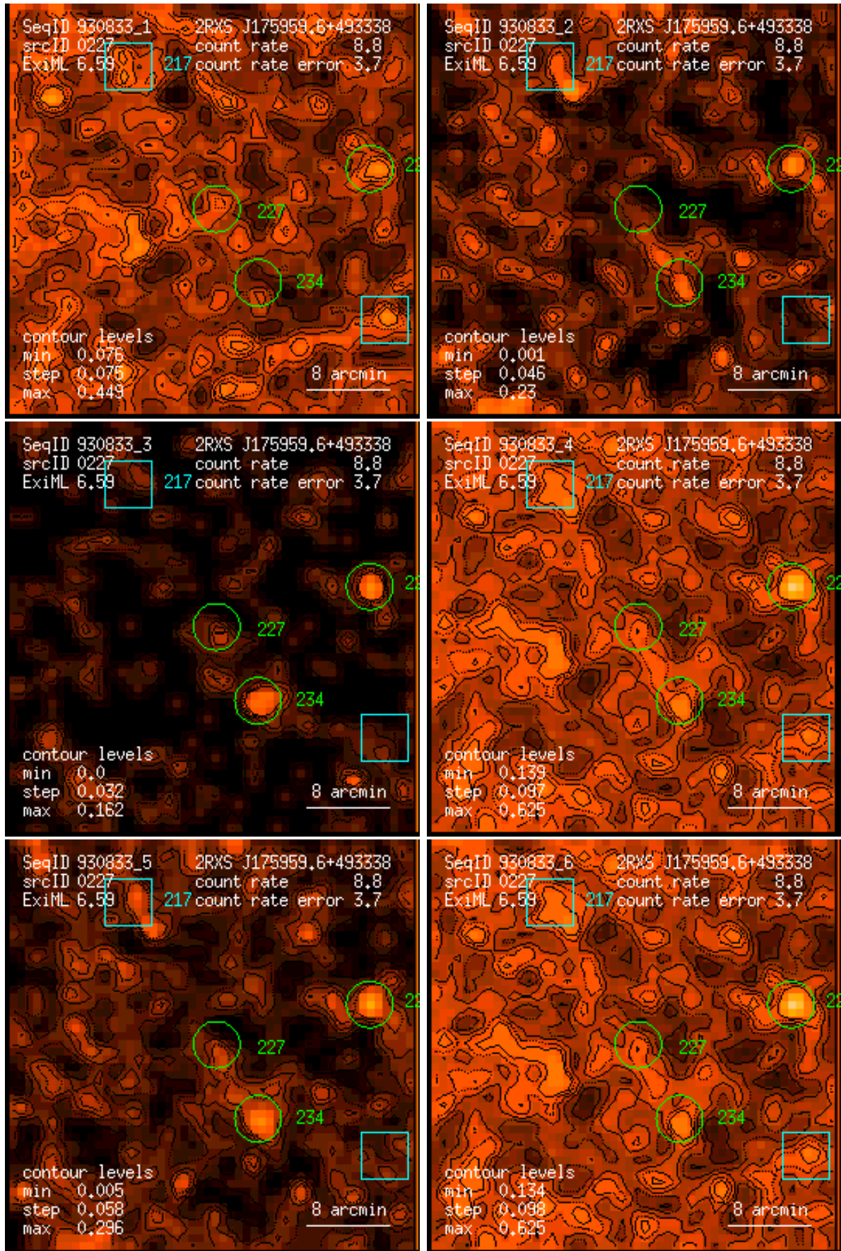
Figure 227: RASS 930833: detection 0227: band rate images, Gaussian filter: (1) PSPC channels 11 – 41, (2) 52 – 90, (3) 91 – 201, (4) 11 – 235, (5) 52 – 201, (6) 11 – 201. Broad band rates in counts/ks. Band rate contour levels in counts/ks/arcmin 2 .
