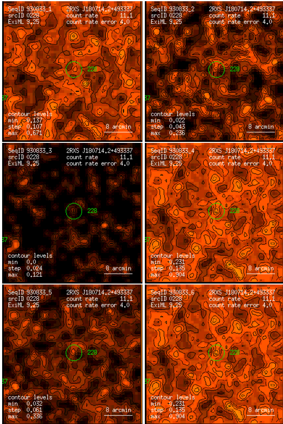
Figure 228: RASS 930833: detection 0228: band rate images, Gaussian filter: (1) PSPC channels 11 – 41, (2) 52 – 90, (3) 91 – 201, (4) 11 – 235, (5) 52 – 201, (6) 11 – 201. Broad band rates in counts/ks. Band rate contour levels in counts/ks/arcmin 2 .
