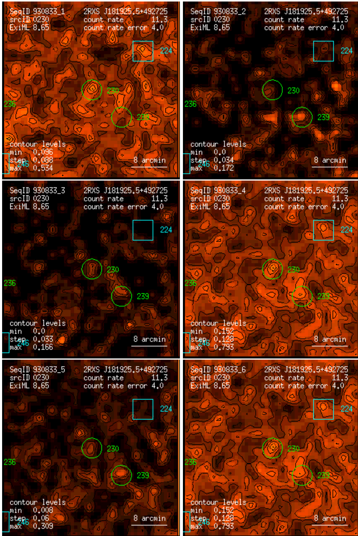
Figure 230: RASS 930833: detection 0230: band rate images, Gaussian filter: (1) PSPC channels 11 – 41, (2) 52 – 90, (3) 91 – 201, (4) 11 – 235, (5) 52 – 201, (6) 11 – 201. Broad band rates in counts/ks. Band rate contour levels in counts/ks/arcmin 2 .
