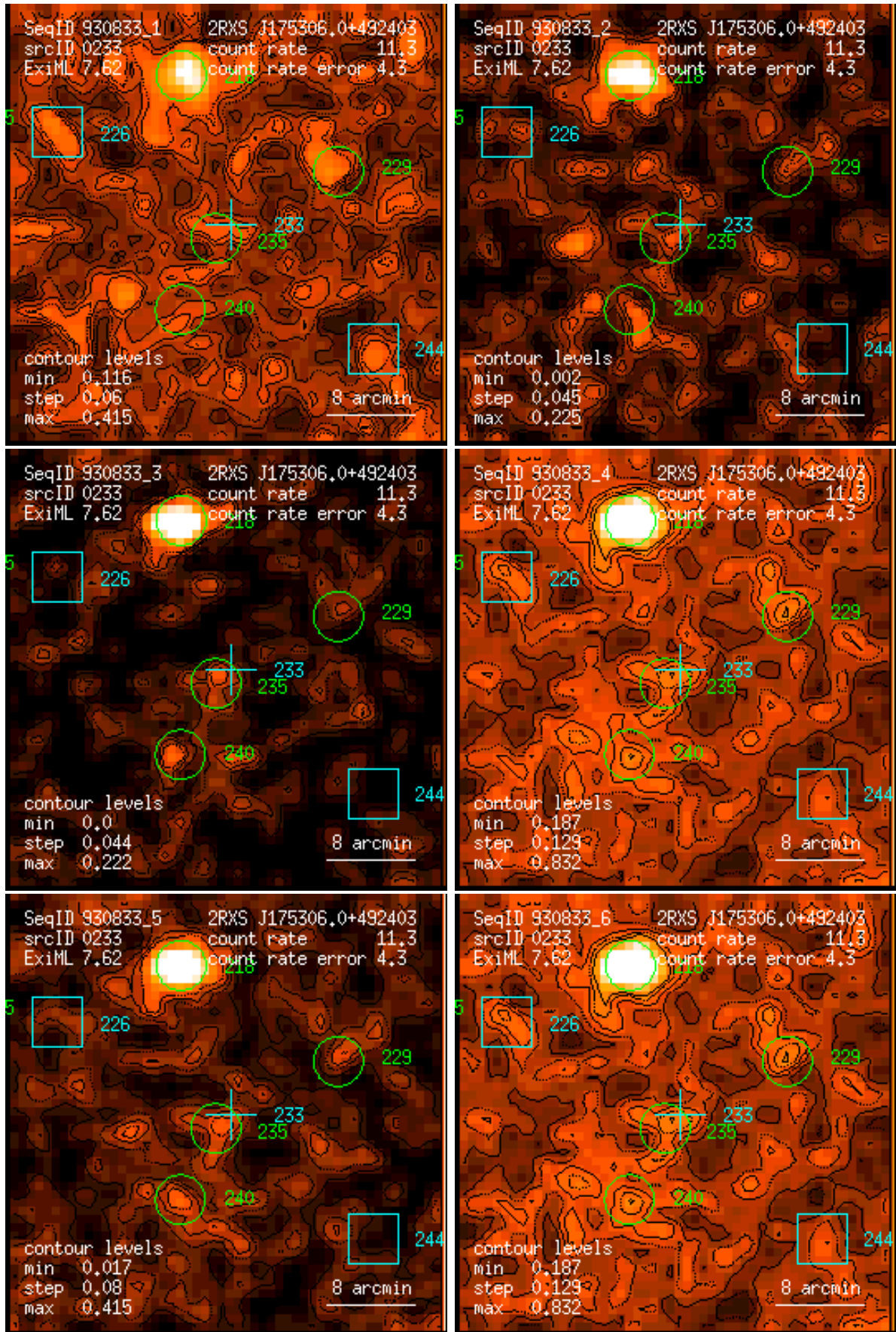
Figure 233: RASS 930833: detection 0233: band rate images, Gaussian filter: (1) PSPC channels 11 – 41, (2) 52 – 90, (3) 91 – 201, (4) 11 – 235, (5) 52 – 201, (6) 11 – 201. Broad band rates in counts/ks. Band rate contour levels in counts/ks/arcmin 2 .
