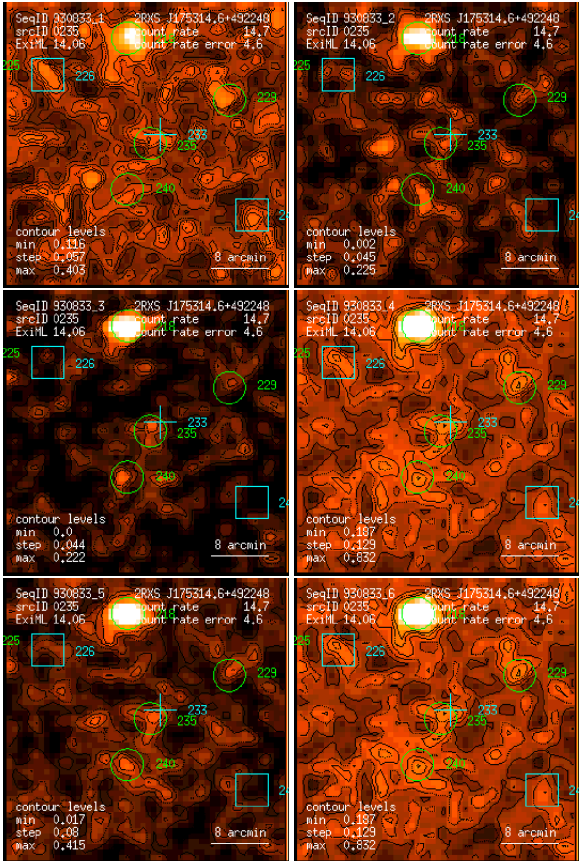
Figure 235: RASS 930833: detection 0235: band rate images, Gaussian filter: (1) PSPC channels 11 – 41, (2) 52 – 90, (3) 91 – 201, (4) 11 – 235, (5) 52 – 201, (6) 11 – 201. Broad band rates in counts/ks. Band rate contour levels in counts/ks/arcmin 2 .
