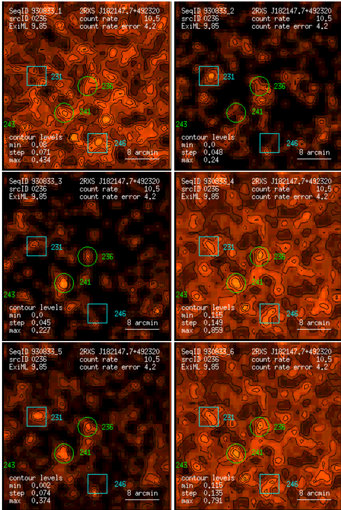
Figure 236: RASS 930833: detection 0236: band rate images, Gaussian filter: (1) PSPC channels 11 – 41, (2) 52 – 90, (3) 91 – 201, (4) 11 – 235, (5) 52 – 201, (6) 11 – 201. Broad band rates in counts/ks. Band rate contour levels in counts/ks/arcmin 2 .
