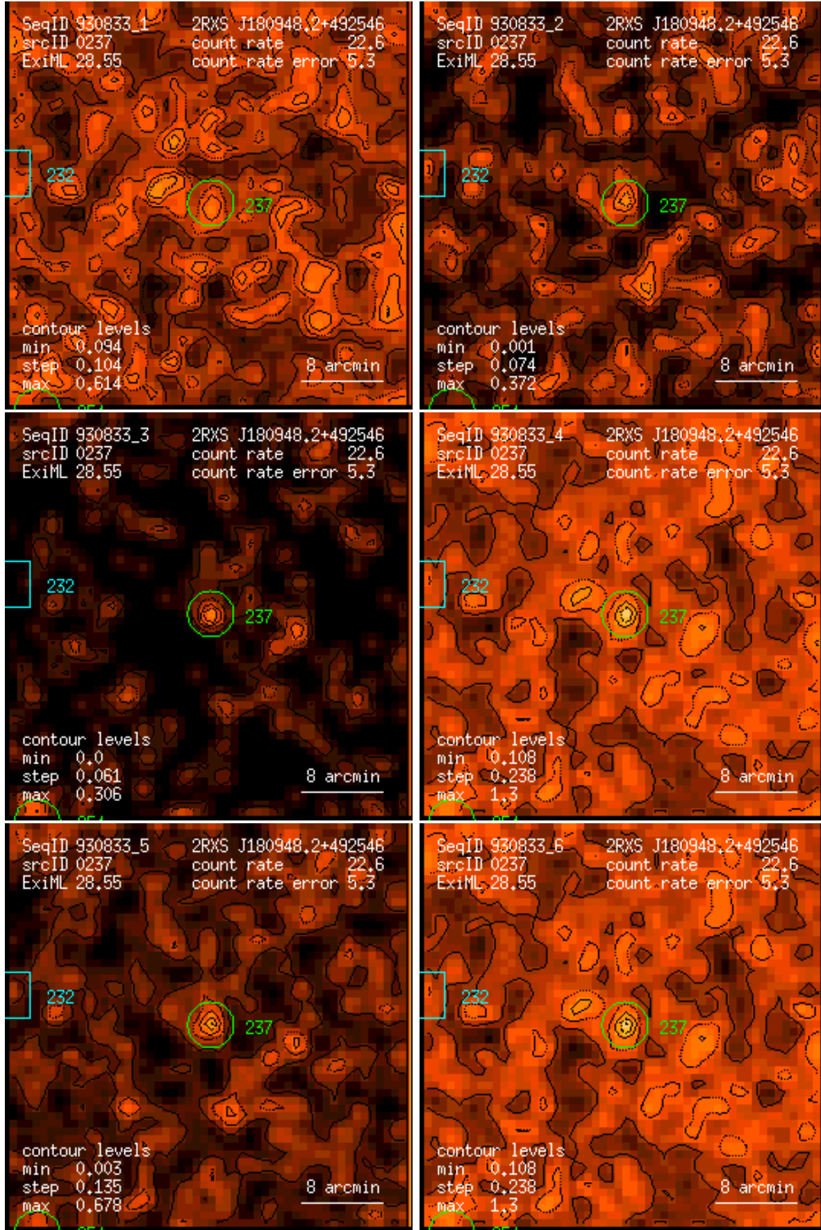
Figure 237: RASS 930833: detection 0237: band rate images, Gaussian filter: (1) PSPC channels 11 – 41, (2) 52 – 90, (3) 91 – 201, (4) 11 – 235, (5) 52 – 201, (6) 11 – 201. Broad band rates in counts/ks. Band rate contour levels in counts/ks/arcmin 2 .
