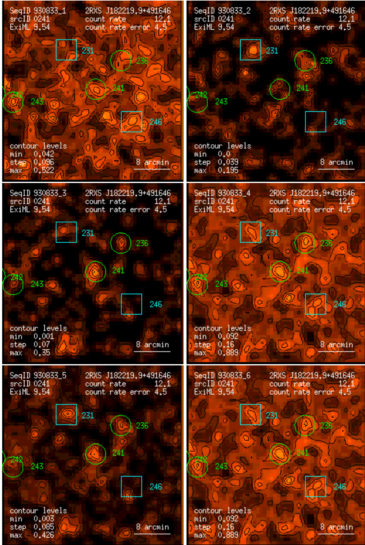
Figure 241: RASS 930833: detection 0241: band rate images, Gaussian filter: (1) PSPC channels 11 – 41, (2) 52 – 90, (3) 91 – 201, (4) 11 – 235, (5) 52 – 201, (6) 11 – 201. Broad band rates in counts/ks. Band rate contour levels in counts/ks/arcmin 2 .
