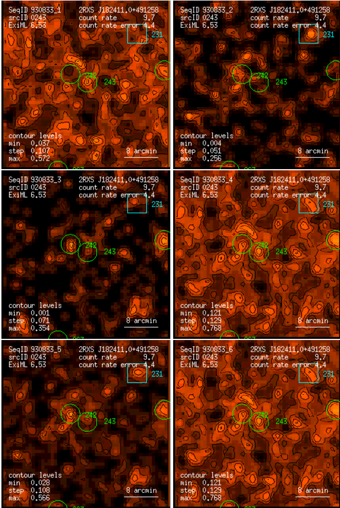
Figure 243: RASS 930833: detection 0243: band rate images, Gaussian filter: (1) PSPC channels 11 – 41, (2) 52 – 90, (3) 91 – 201, (4) 11 – 235, (5) 52 – 201, (6) 11 – 201. Broad band rates in counts/ks. Band rate contour levels in counts/ks/arcmin 2 .
