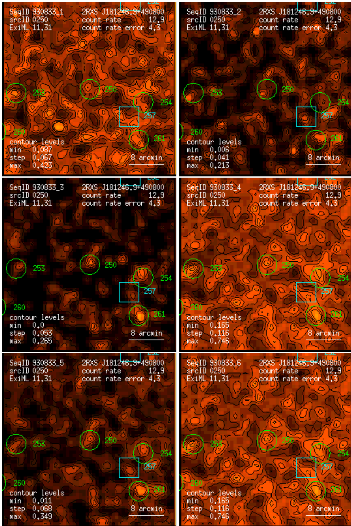
Figure 250: RASS 930833: detection 0250: band rate images, Gaussian filter: (1) PSPC channels 11 – 41, (2) 52 – 90, (3) 91 – 201, (4) 11 – 235, (5) 52 – 201, (6) 11 – 201. Broad band rates in counts/ks. Band rate contour levels in counts/ks/arcmin 2 .
