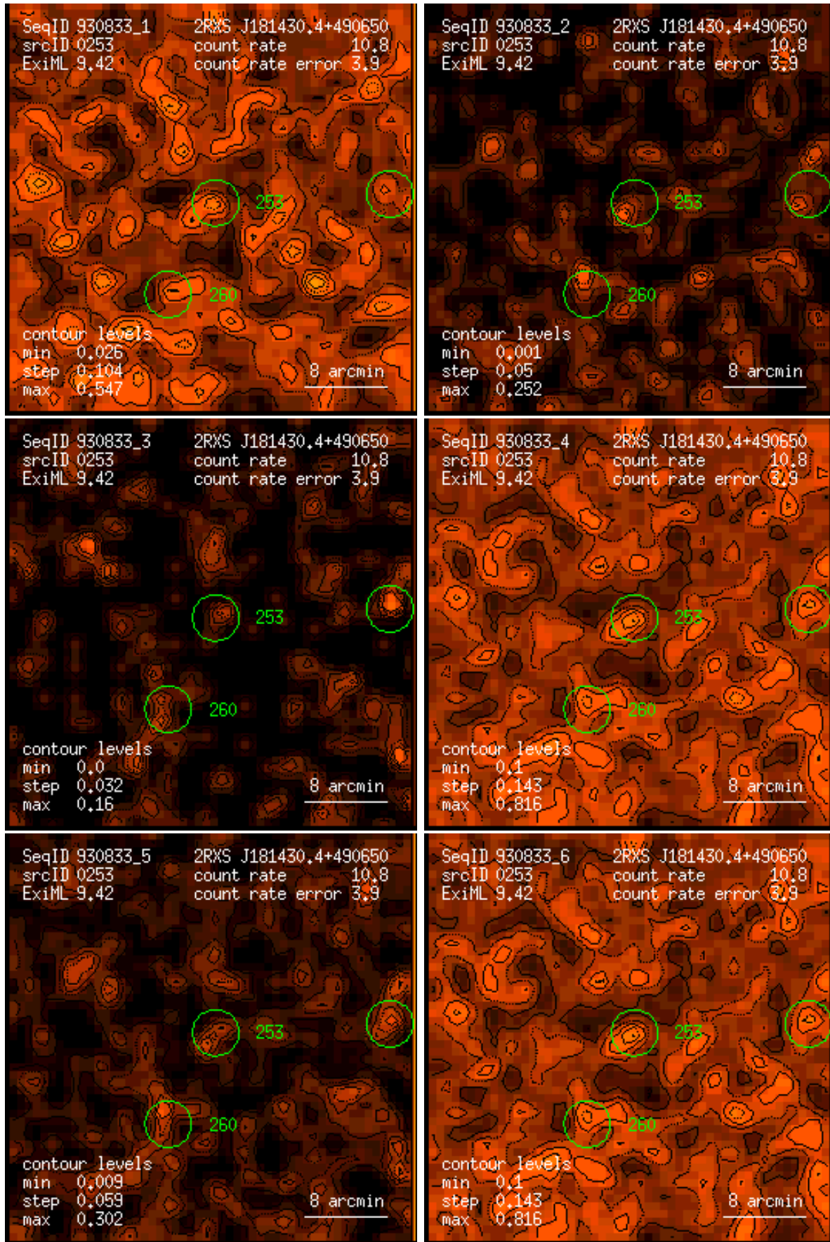
Figure 253: RASS 930833: detection 0253: band rate images, Gaussian filter: (1) PSPC channels 11 – 41, (2) 52 – 90, (3) 91 – 201, (4) 11 – 235, (5) 52 – 201, (6) 11 – 201. Broad band rates in counts/ks. Band rate contour levels in counts/ks/arcmin 2 .
