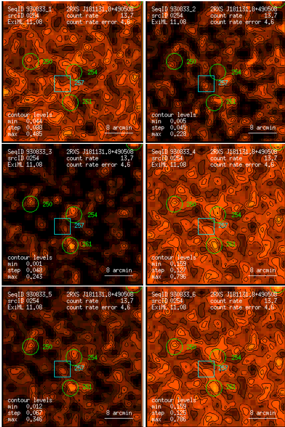
Figure 254: RASS 930833: detection 0254: band rate images, Gaussian filter: (1) PSPC channels 11 – 41, (2) 52 – 90, (3) 91 – 201, (4) 11 – 235, (5) 52 – 201, (6) 11 – 201. Broad band rates in counts/ks. Band rate contour levels in counts/ks/arcmin 2 .
