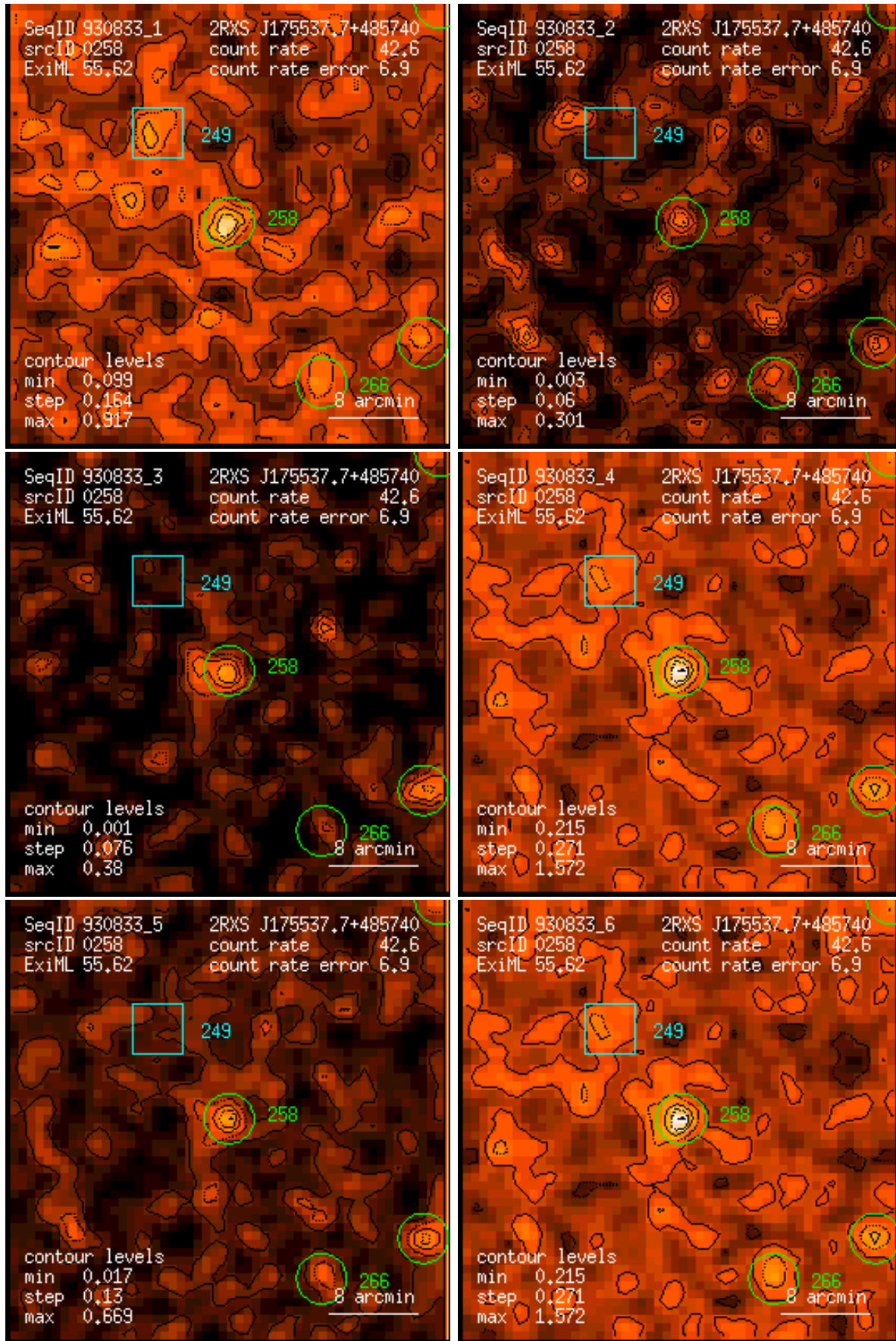
Figure 258: RASS 930833: detection 0258: band rate images, Gaussian filter: (1) PSPC channels 11 – 41, (2) 52 – 90, (3) 91 – 201, (4) 11 – 235, (5) 52 – 201, (6) 11 – 201. Broad band rates in counts/ks. Band rate contour levels in counts/ks/arcmin 2 .
