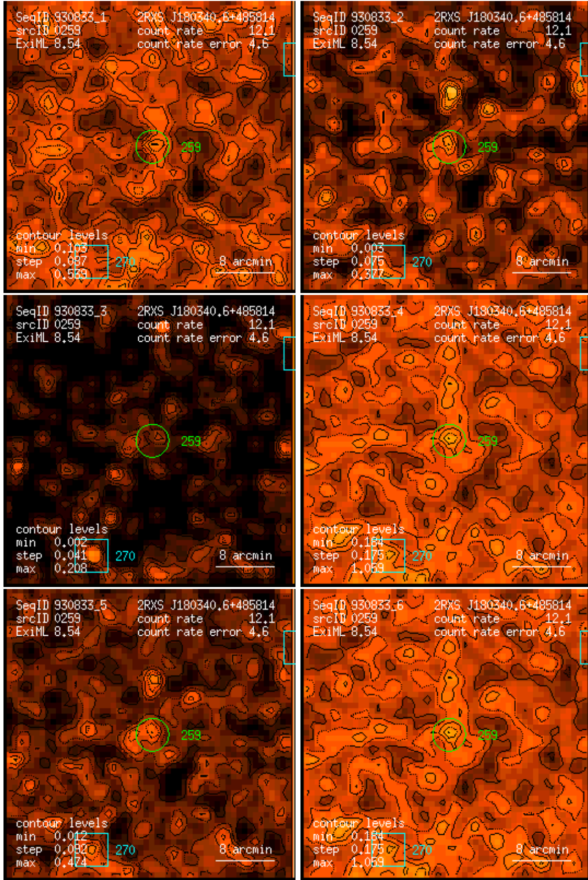
Figure 259: RASS 930833: detection 0259: band rate images, Gaussian filter: (1) PSPC channels 11 – 41, (2) 52 – 90, (3) 91 – 201, (4) 11 – 235, (5) 52 – 201, (6) 11 – 201. Broad band rates in counts/ks. Band rate contour levels in counts/ks/arcmin 2 .
