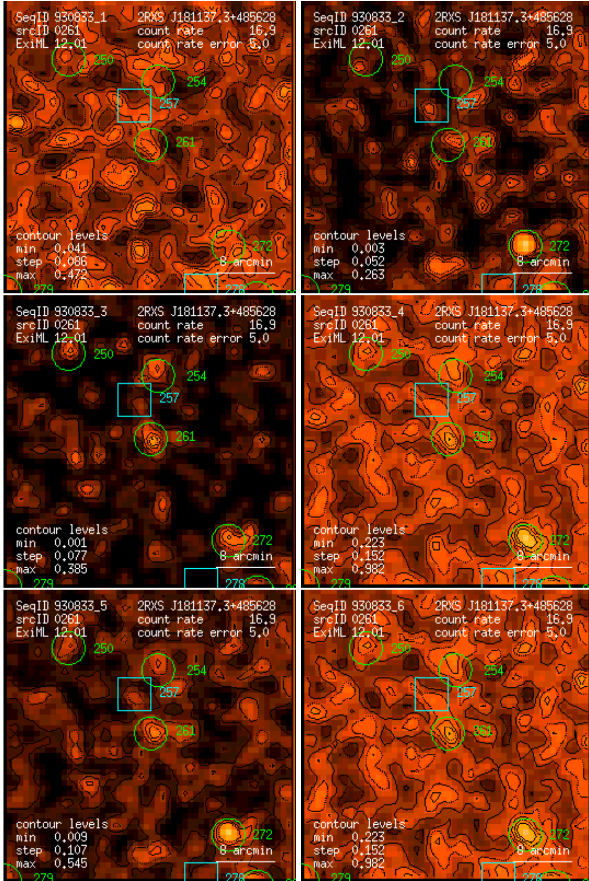
Figure 261: RASS 930833: detection 0261: band rate images, Gaussian filter: (1) PSPC channels 11 – 41, (2) 52 – 90, (3) 91 – 201, (4) 11 – 235, (5) 52 – 201, (6) 11 – 201. Broad band rates in counts/ks. Band rate contour levels in counts/ks/arcmin 2 .
