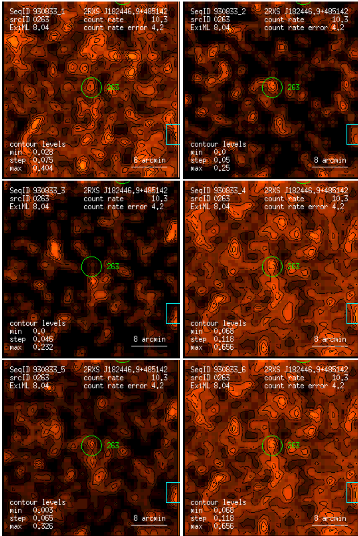
Figure 263: RASS 930833: detection 0263: band rate images, Gaussian filter: (1) PSPC channels 11 – 41, (2) 52 – 90, (3) 91 – 201, (4) 11 – 235, (5) 52 – 201, (6) 11 – 201. Broad band rates in counts/ks. Band rate contour levels in counts/ks/arcmin 2 .
