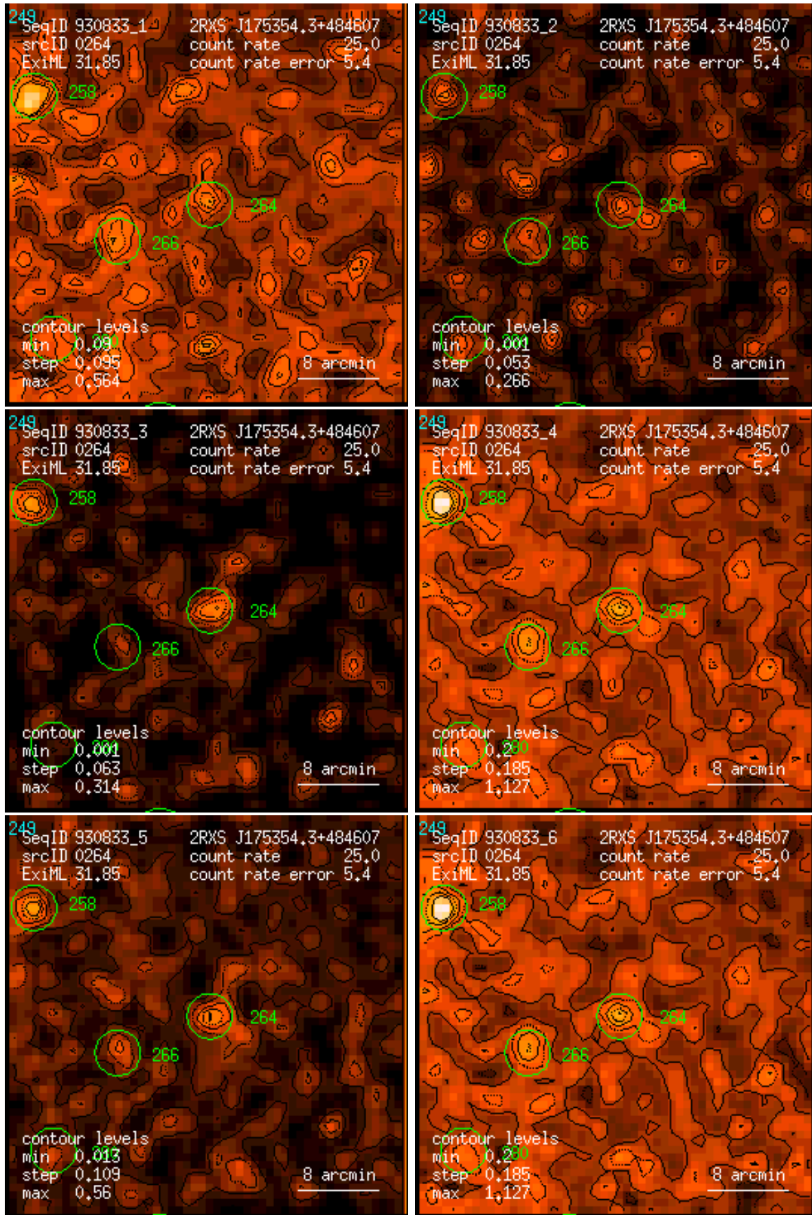
Figure 264: RASS 930833: detection 0264: band rate images, Gaussian filter: (1) PSPC channels 11 – 41, (2) 52 – 90, (3) 91 – 201, (4) 11 – 235, (5) 52 – 201, (6) 11 – 201. Broad band rates in counts/ks. Band rate contour levels in counts/ks/arcmin 2 .
