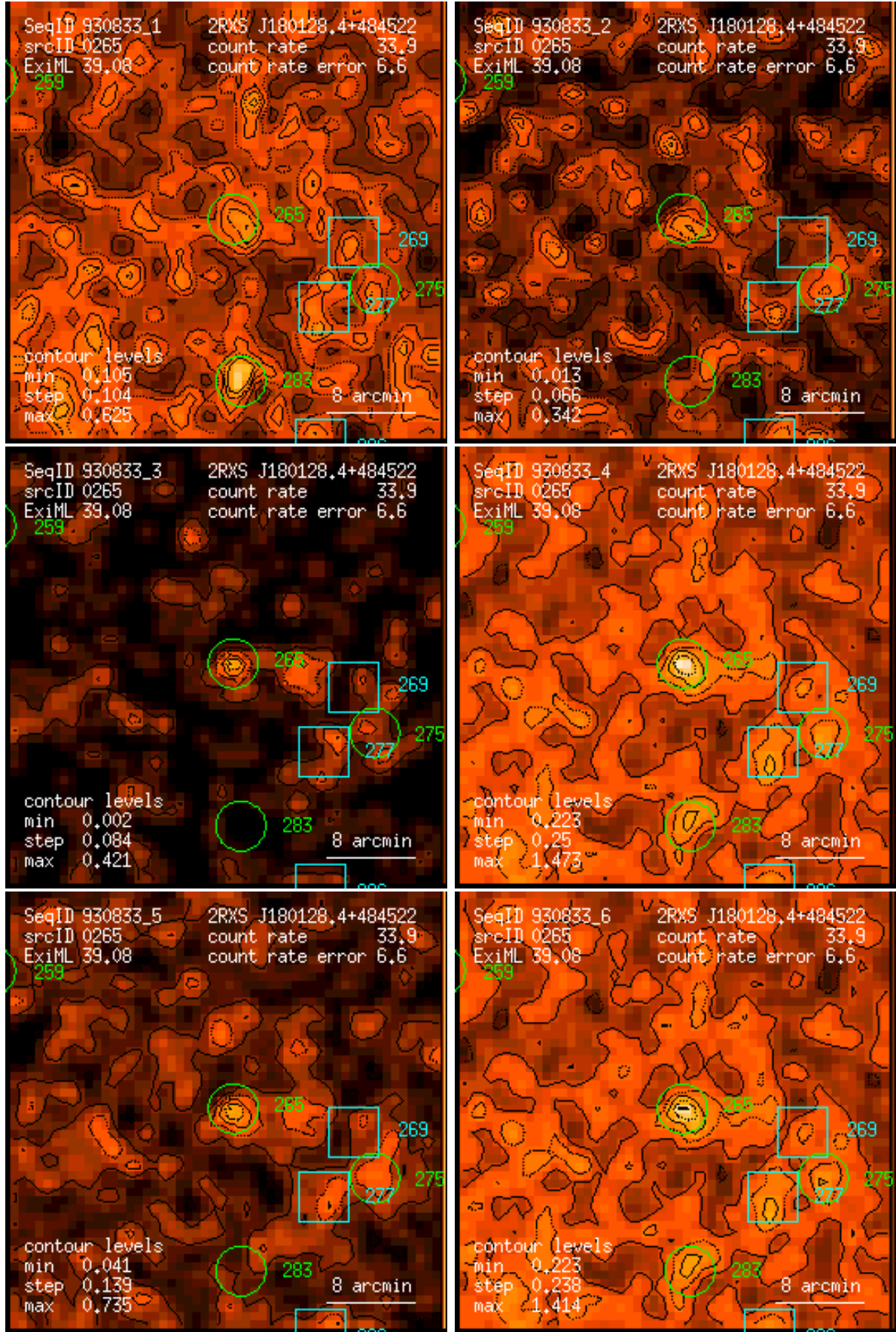
Figure 265: RASS 930833: detection 0265: band rate images, Gaussian filter: (1) PSPC channels 11 – 41, (2) 52 – 90, (3) 91 – 201, (4) 11 – 235, (5) 52 – 201, (6) 11 – 201. Broad band rates in counts/ks. Band rate contour levels in counts/ks/arcmin 2 .
