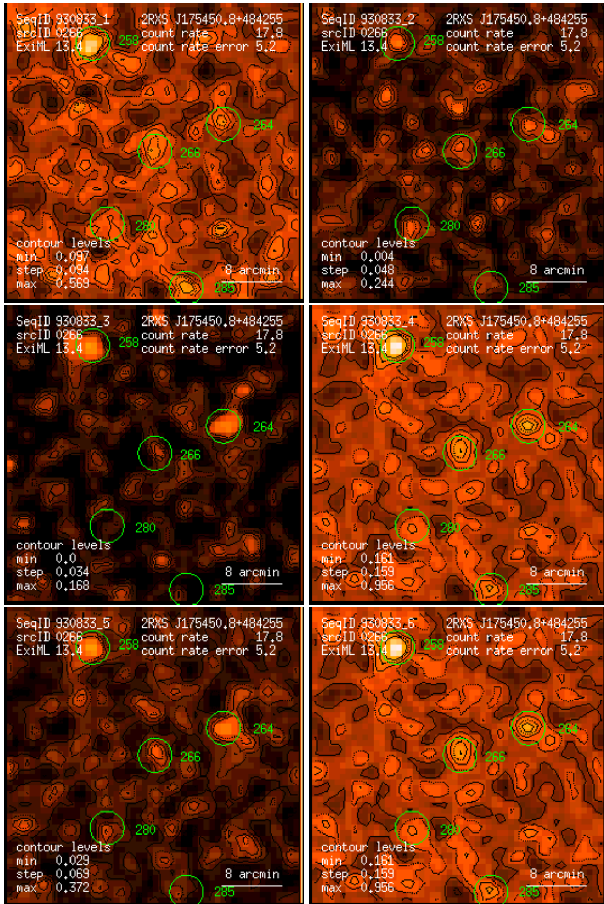
Figure 266: RASS 930833: detection 0266: band rate images, Gaussian filter: (1) PSPC channels 11 – 41, (2) 52 – 90, (3) 91 – 201, (4) 11 – 235, (5) 52 – 201, (6) 11 – 201. Broad band rates in counts/ks. Band rate contour levels in counts/ks/arcmin 2 .
