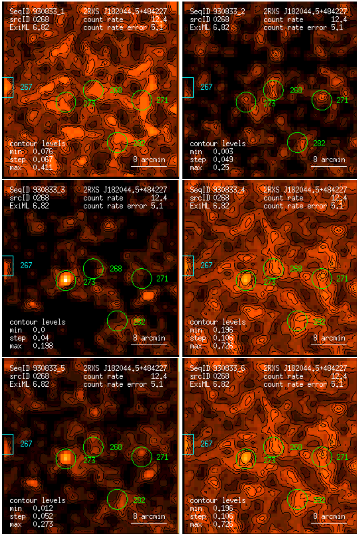
Figure 268: RASS 930833: detection 0268: band rate images, Gaussian filter: (1) PSPC channels 11 – 41, (2) 52 – 90, (3) 91 – 201, (4) 11 – 235, (5) 52 – 201, (6) 11 – 201. Broad band rates in counts/ks. Band rate contour levels in counts/ks/arcmin 2 .
