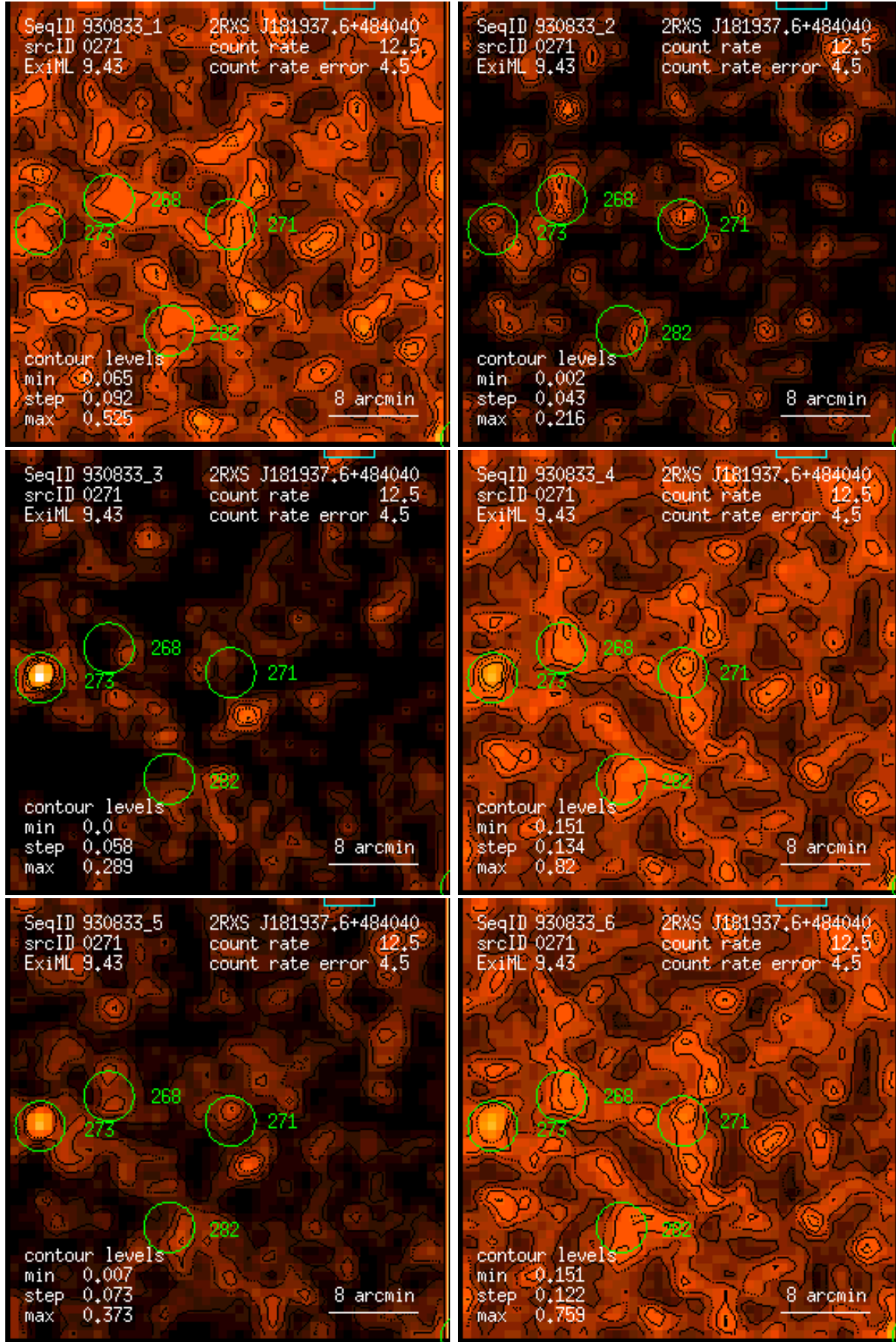
Figure 271: RASS 930833: detection 0271: band rate images, Gaussian filter: (1) PSPC channels 11 – 41, (2) 52 – 90, (3) 91 – 201, (4) 11 – 235, (5) 52 – 201, (6) 11 – 201. Broad band rates in counts/ks. Band rate contour levels in counts/ks/arcmin 2 .
