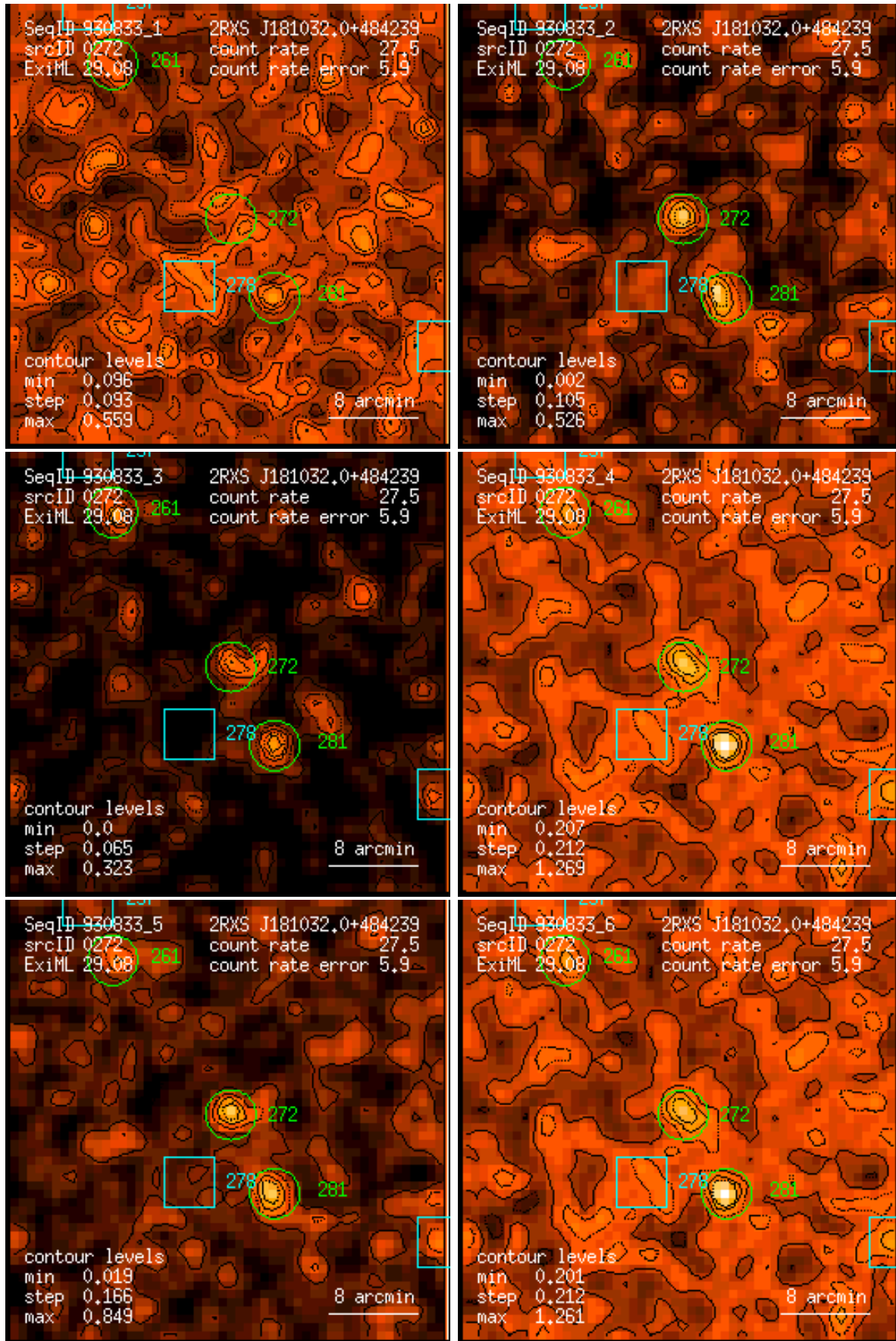
Figure 272: RASS 930833: detection 0272: band rate images, Gaussian filter: (1) PSPC channels 11 – 41, (2) 52 – 90, (3) 91 – 201, (4) 11 – 235, (5) 52 – 201, (6) 11 – 201. Broad band rates in counts/ks. Band rate contour levels in counts/ks/arcmin 2 .
