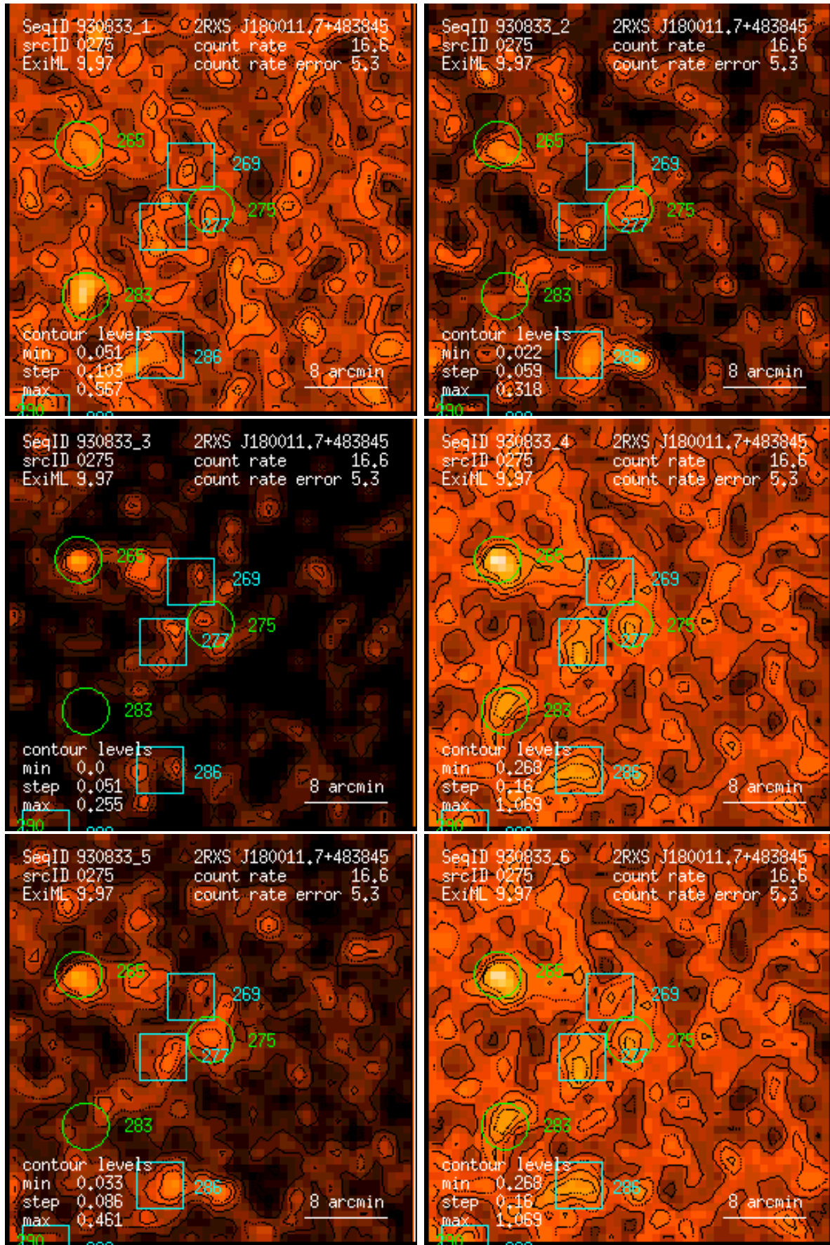
Figure 275: RASS 930833: detection 0275: band rate images, Gaussian filter: (1) PSPC channels 11 – 41, (2) 52 – 90, (3) 91 – 201, (4) 11 – 235, (5) 52 – 201, (6) 11 – 201. Broad band rates in counts/ks. Band rate contour levels in counts/ks/arcmin 2 .
