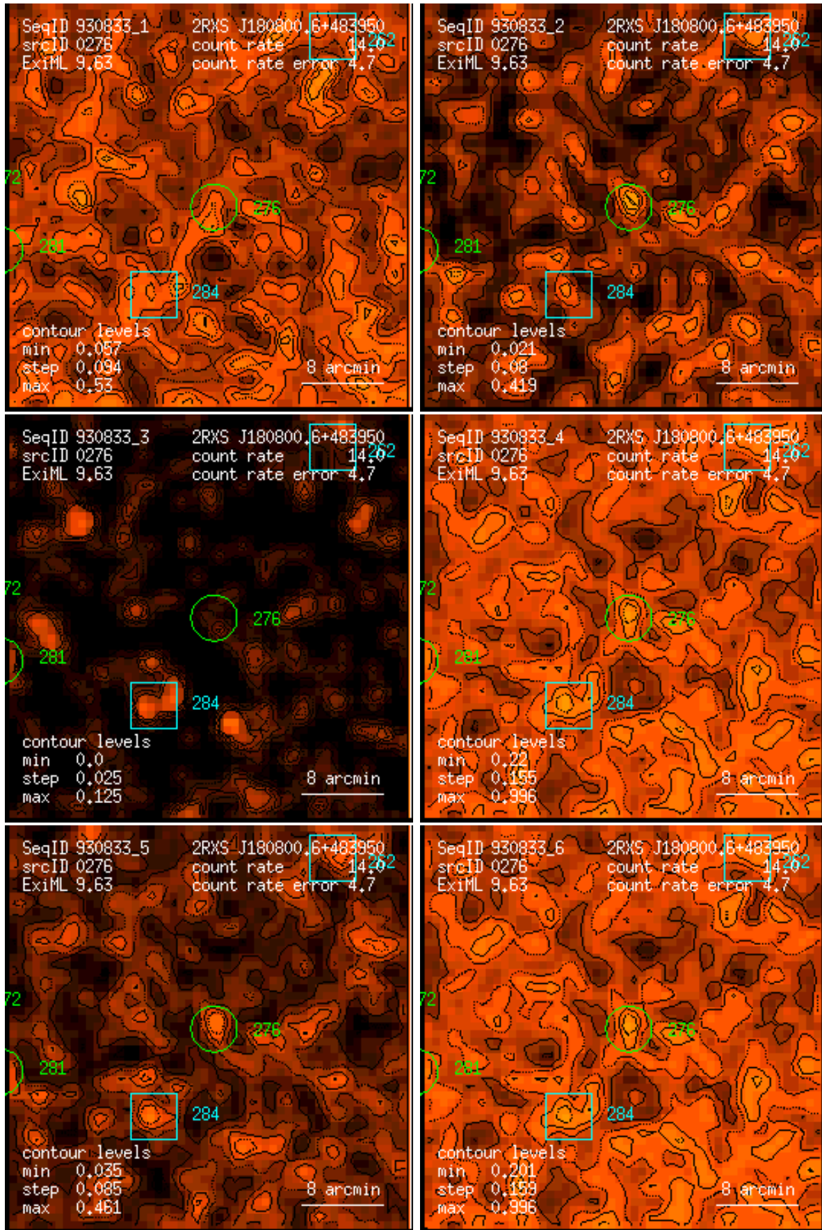
Figure 276: RASS 930833: detection 0276: band rate images, Gaussian filter: (1) PSPC channels 11 – 41, (2) 52 – 90, (3) 91 – 201, (4) 11 – 235, (5) 52 – 201, (6) 11 – 201. Broad band rates in counts/ks. Band rate contour levels in counts/ks/arcmin 2 .
