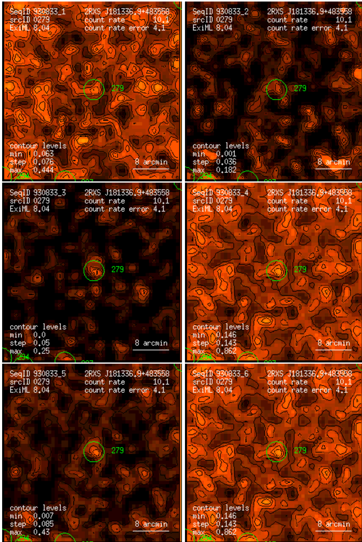
Figure 279: RASS 930833: detection 0279: band rate images, Gaussian filter: (1) PSPC channels 11 – 41, (2) 52 – 90, (3) 91 – 201, (4) 11 – 235, (5) 52 – 201, (6) 11 – 201. Broad band rates in counts/ks. Band rate contour levels in counts/ks/arcmin 2 .
