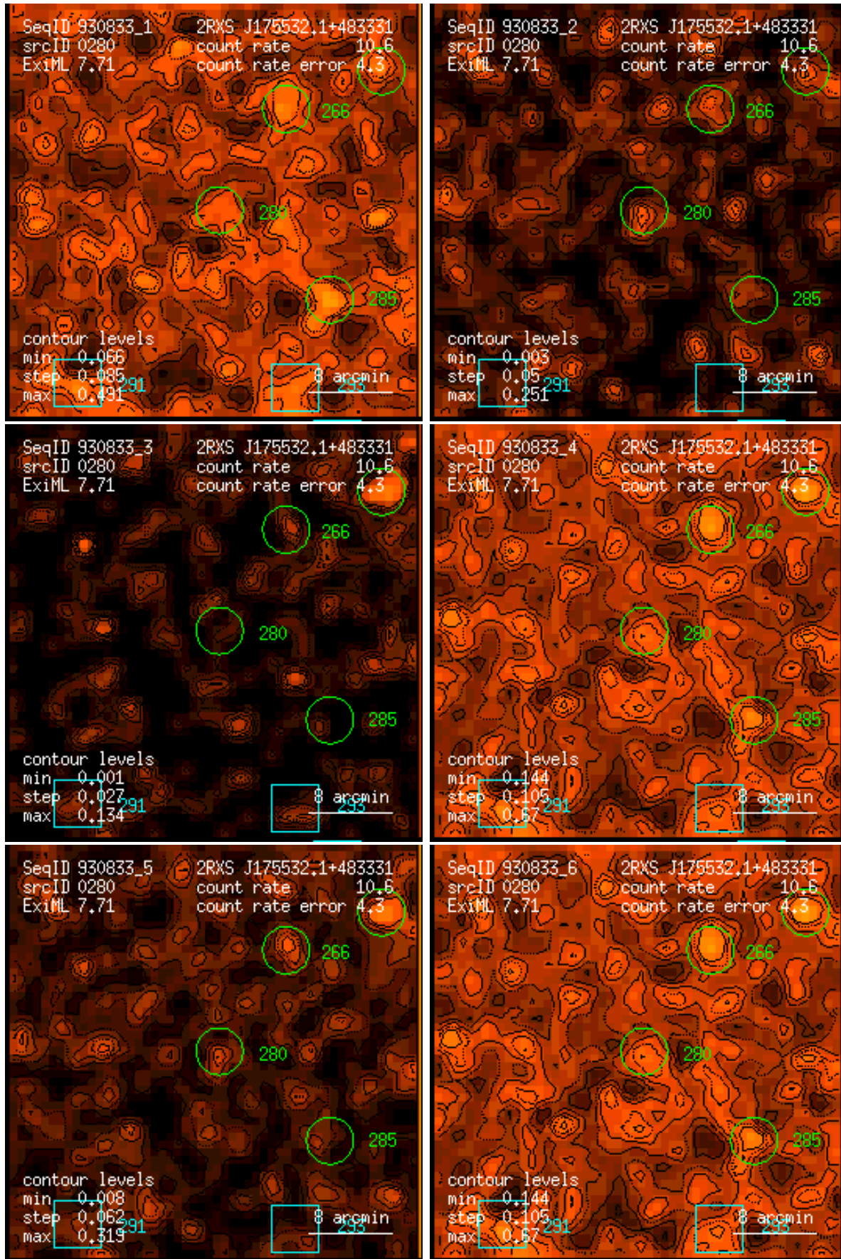
Figure 280: RASS 930833: detection 0280: band rate images, Gaussian filter: (1) PSPC channels 11 – 41, (2) 52 – 90, (3) 91 – 201, (4) 11 – 235, (5) 52 – 201, (6) 11 – 201. Broad band rates in counts/ks. Band rate contour levels in counts/ks/arcmin 2 .
