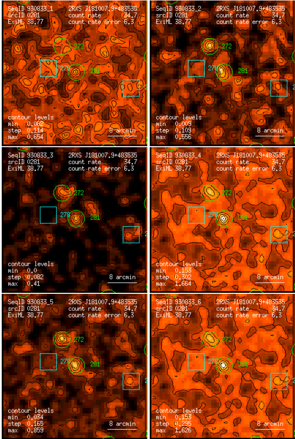
Figure 281: RASS 930833: detection 0281: band rate images, Gaussian filter: (1) PSPC channels 11 – 41, (2) 52 – 90, (3) 91 – 201, (4) 11 – 235, (5) 52 – 201, (6) 11 – 201. Broad band rates in counts/ks. Band rate contour levels in counts/ks/arcmin 2 .
