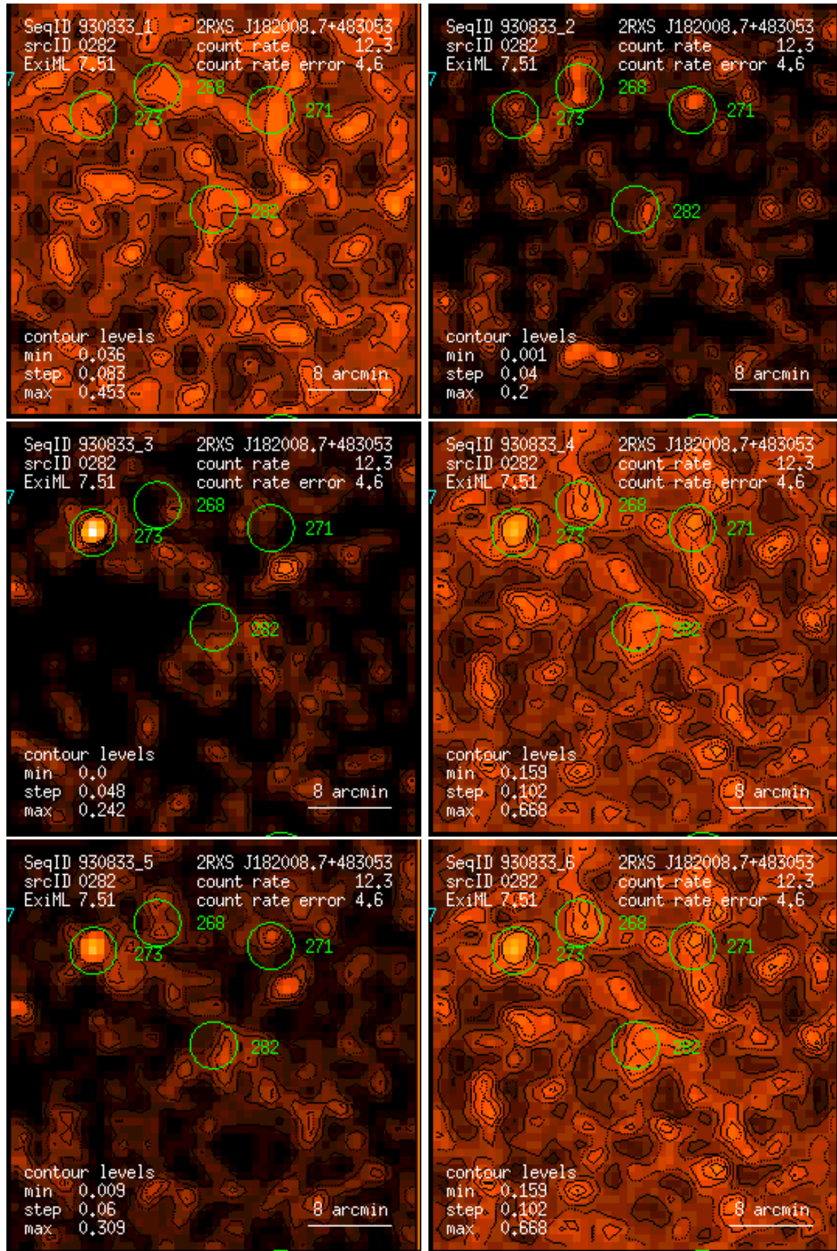
Figure 282: RASS 930833: detection 0282: band rate images, Gaussian filter: (1) PSPC channels 11 – 41, (2) 52 – 90, (3) 91 – 201, (4) 11 – 235, (5) 52 – 201, (6) 11 – 201. Broad band rates in counts/ks. Band rate contour levels in counts/ks/arcmin 2 .
