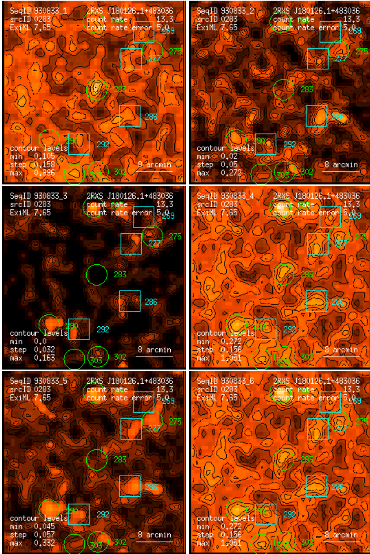
Figure 283: RASS 930833: detection 0283: band rate images, Gaussian filter: (1) PSPC channels 11 – 41, (2) 52 – 90, (3) 91 – 201, (4) 11 – 235, (5) 52 – 201, (6) 11 – 201. Broad band rates in counts/ks. Band rate contour levels in counts/ks/arcmin 2 .
