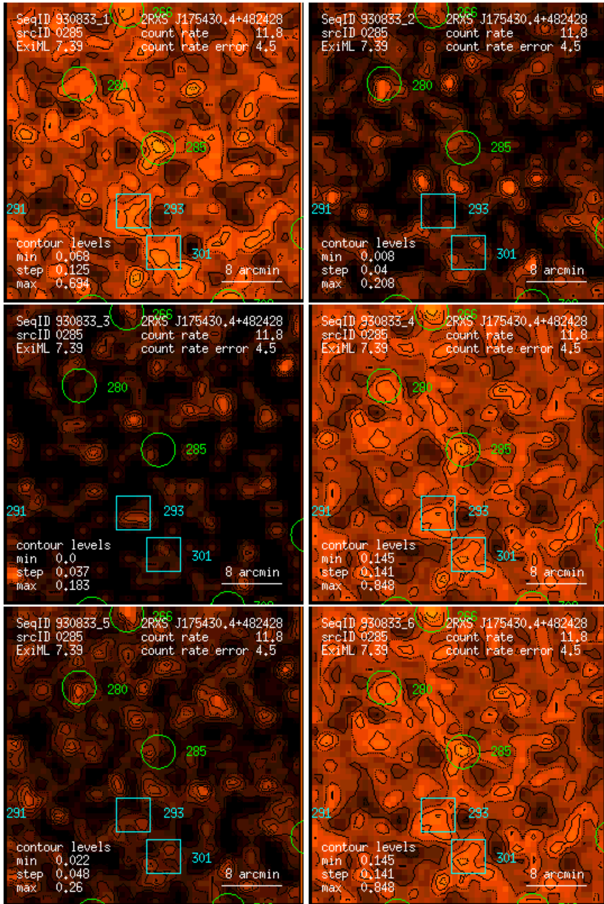
Figure 285: RASS 930833: detection 0285: band rate images, Gaussian filter: (1) PSPC channels 11 – 41, (2) 52 – 90, (3) 91 – 201, (4) 11 – 235, (5) 52 – 201, (6) 11 – 201. Broad band rates in counts/ks. Band rate contour levels in counts/ks/arcmin 2 .
