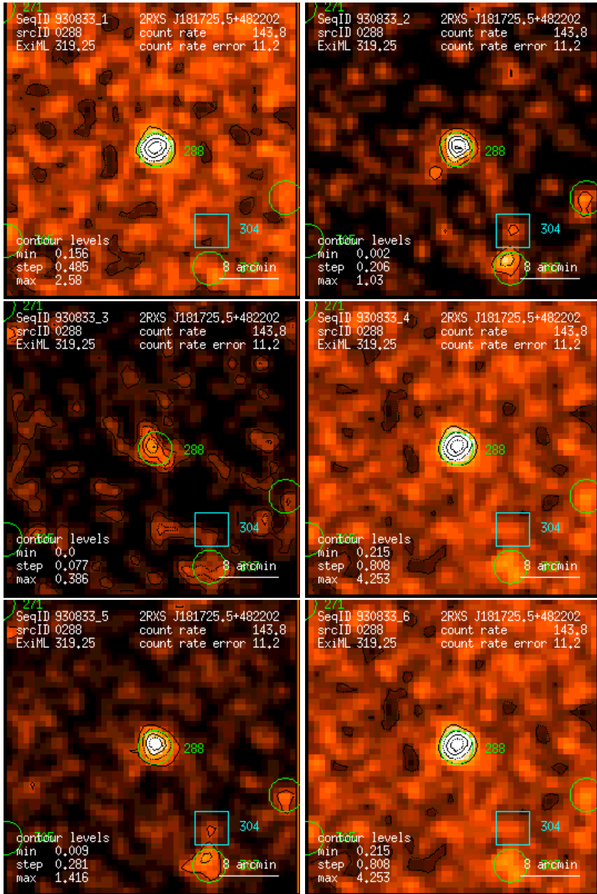
Figure 288: RASS 930833: detection 0288: band rate images, Gaussian filter: (1) PSPC channels 11 – 41, (2) 52 – 90, (3) 91 – 201, (4) 11 – 235, (5) 52 – 201, (6) 11 – 201. Broad band rates in counts/ks. Band rate contour levels in counts/ks/arcmin 2 .
